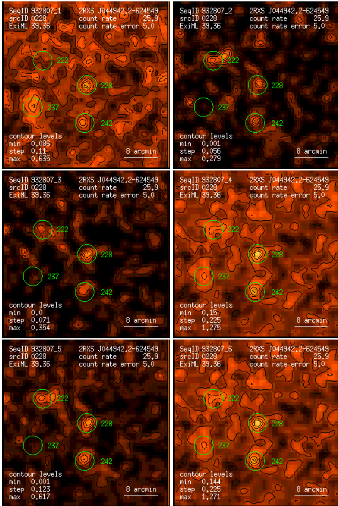
Figure 228: RASS 932807: detection 0228: band rate images, Gaussian filter: (1) PSPC channels 11 – 41, (2) 52 – 90, (3) 91 – 201, (4) 11 – 235, (5) 52 – 201, (6) 11 – 201. Broad band rates in counts/ks. Band rate contour levels in counts/ks/arcmin 2 .
