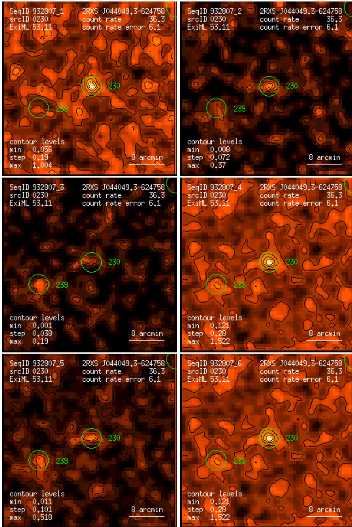
Figure 230: RASS 932807: detection 0230: band rate images, Gaussian filter: (1) PSPC channels 11 – 41, (2) 52 – 90, (3) 91 – 201, (4) 11 – 235, (5) 52 – 201, (6) 11 – 201. Broad band rates in counts/ks. Band rate contour levels in counts/ks/arcmin 2 .
