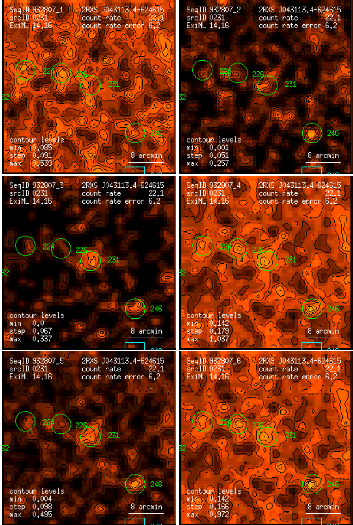
Figure 231: RASS 932807: detection 0231: band rate images, Gaussian filter: (1) PSPC channels 11 – 41, (2) 52 – 90, (3) 91 – 201, (4) 11 – 235, (5) 52 – 201, (6) 11 – 201. Broad band rates in counts/ks. Band rate contour levels in counts/ks/arcmin 2 .
