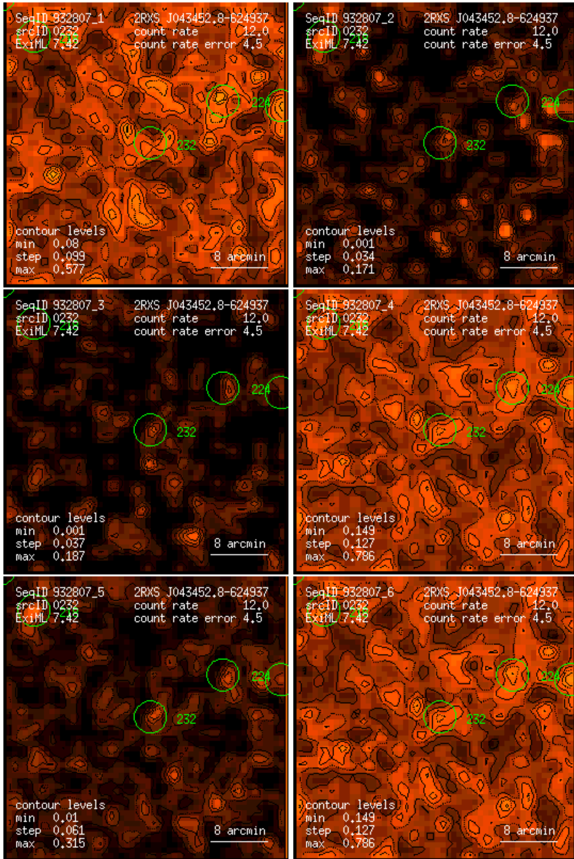
Figure 232: RASS 932807: detection 0232: band rate images, Gaussian filter: (1) PSPC channels 11 – 41, (2) 52 – 90, (3) 91 – 201, (4) 11 – 235, (5) 52 – 201, (6) 11 – 201. Broad band rates in counts/ks. Band rate contour levels in counts/ks/arcmin 2 .
