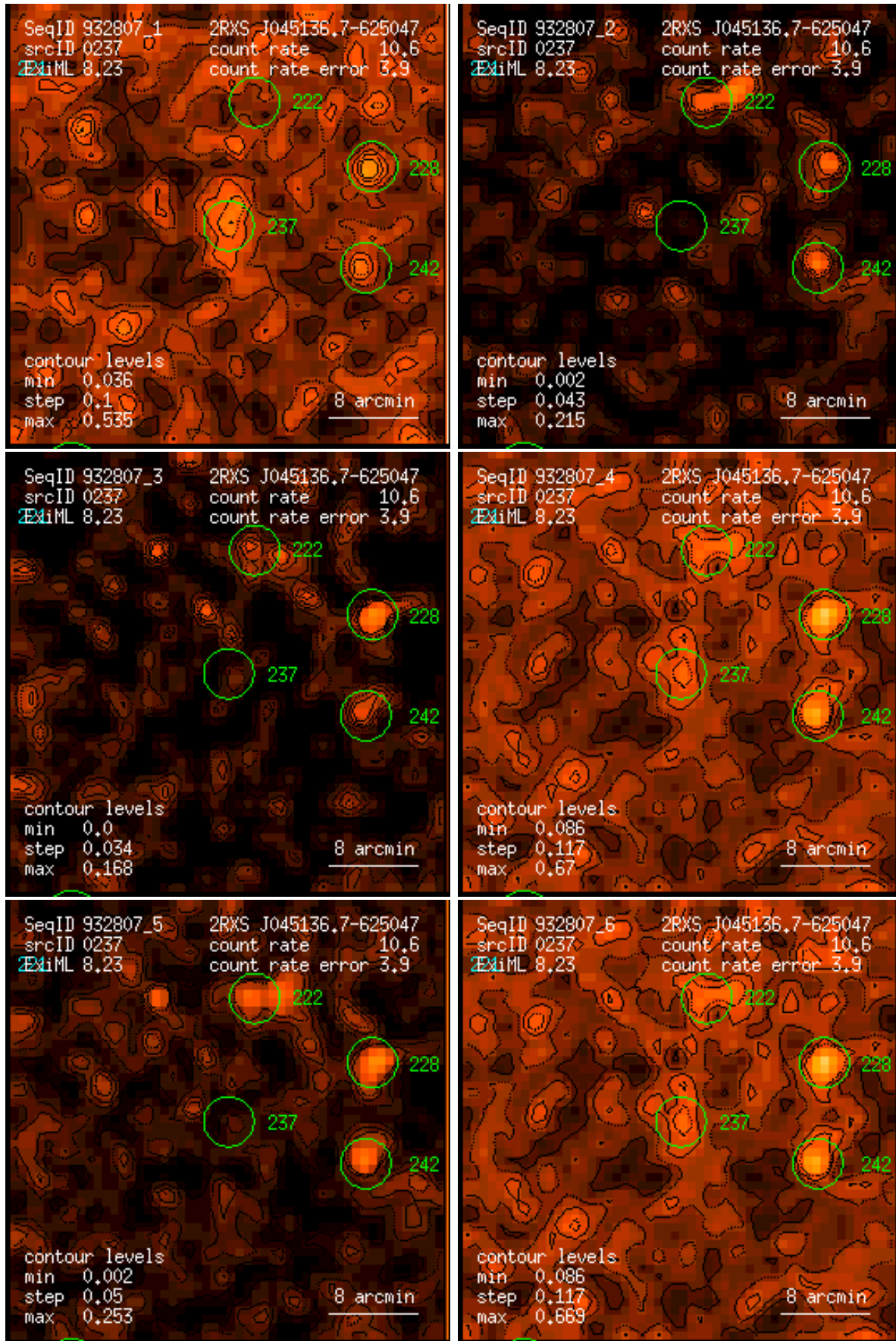
Figure 237: RASS 932807: detection 0237: band rate images, Gaussian filter: (1) PSPC channels 11 – 41, (2) 52 – 90, (3) 91 – 201, (4) 11 – 235, (5) 52 – 201, (6) 11 – 201. Broad band rates in counts/ks. Band rate contour levels in counts/ks/arcmin 2 .
