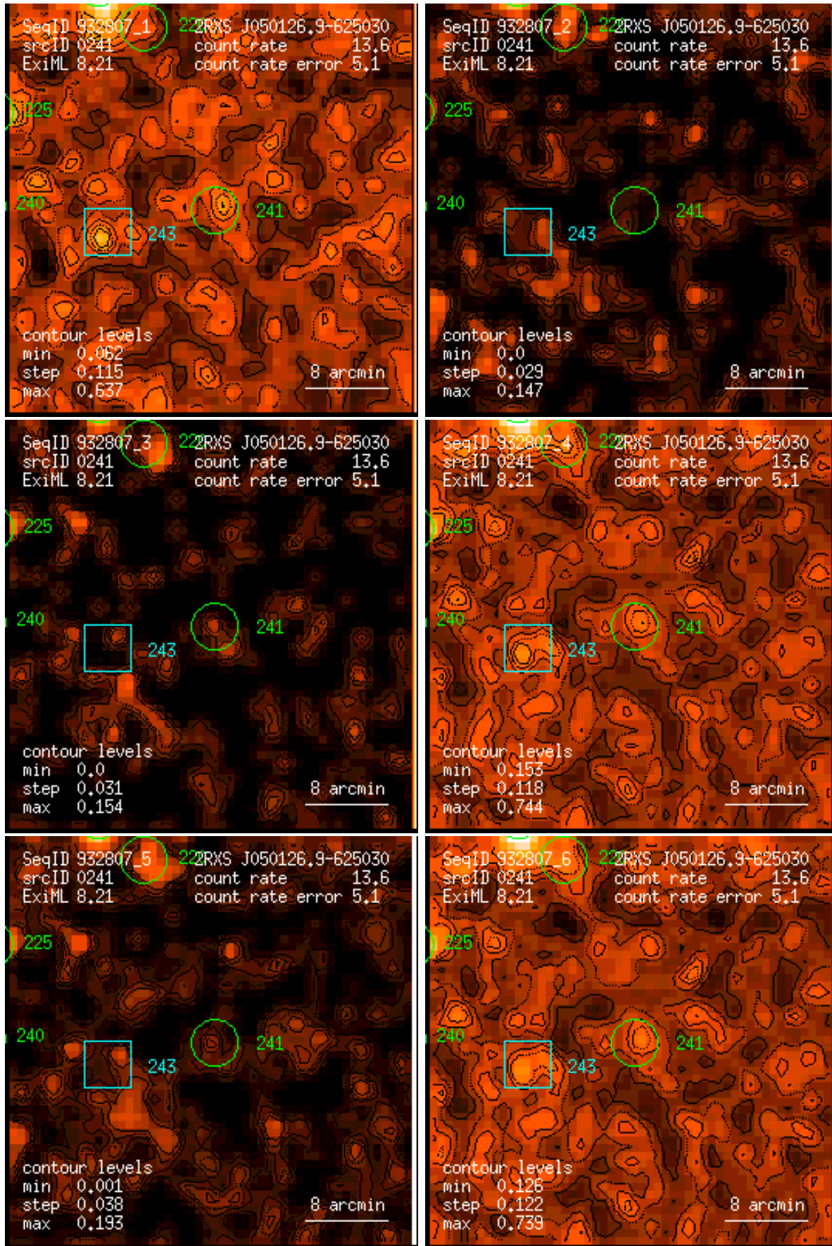
Figure 241: RASS 932807: detection 0241: band rate images, Gaussian filter: (1) PSPC channels 11 – 41, (2) 52 – 90, (3) 91 – 201, (4) 11 – 235, (5) 52 – 201, (6) 11 – 201. Broad band rates in counts/ks. Band rate contour levels in counts/ks/arcmin 2 .
