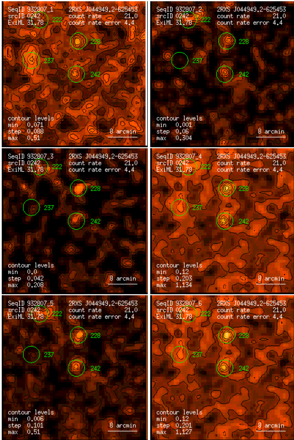
Figure 242: RASS 932807: detection 0242: band rate images, Gaussian filter: (1) PSPC channels 11 – 41, (2) 52 – 90, (3) 91 – 201, (4) 11 – 235, (5) 52 – 201, (6) 11 – 201. Broad band rates in counts/ks. Band rate contour levels in counts/ks/arcmin 2 .
