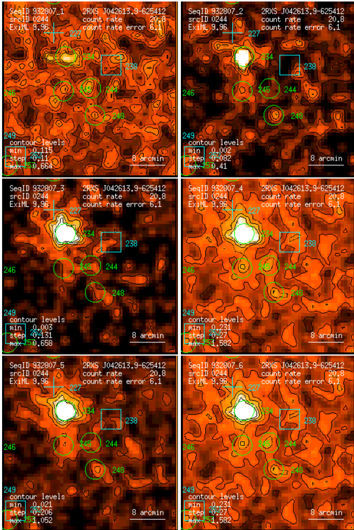
Figure 244: RASS 932807: detection 0244: band rate images, Gaussian filter: (1) PSPC channels 11 – 41, (2) 52 – 90, (3) 91 – 201, (4) 11 – 235, (5) 52 – 201, (6) 11 – 201. Broad band rates in counts/ks. Band rate contour levels in counts/ks/arcmin 2 .
