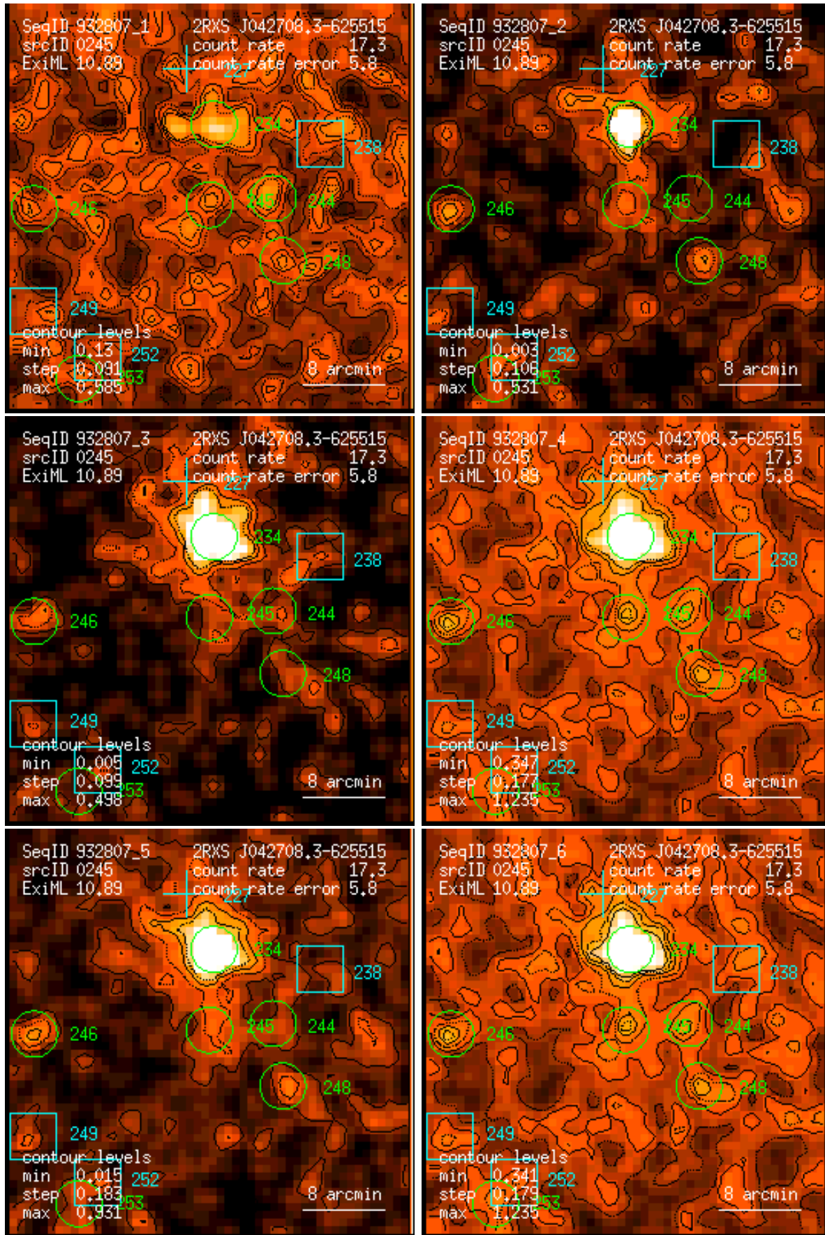
Figure 245: RASS 932807: detection 0245: band rate images, Gaussian filter: (1) PSPC channels 11 – 41, (2) 52 – 90, (3) 91 – 201, (4) 11 – 235, (5) 52 – 201, (6) 11 – 201. Broad band rates in counts/ks. Band rate contour levels in counts/ks/arcmin 2 .
