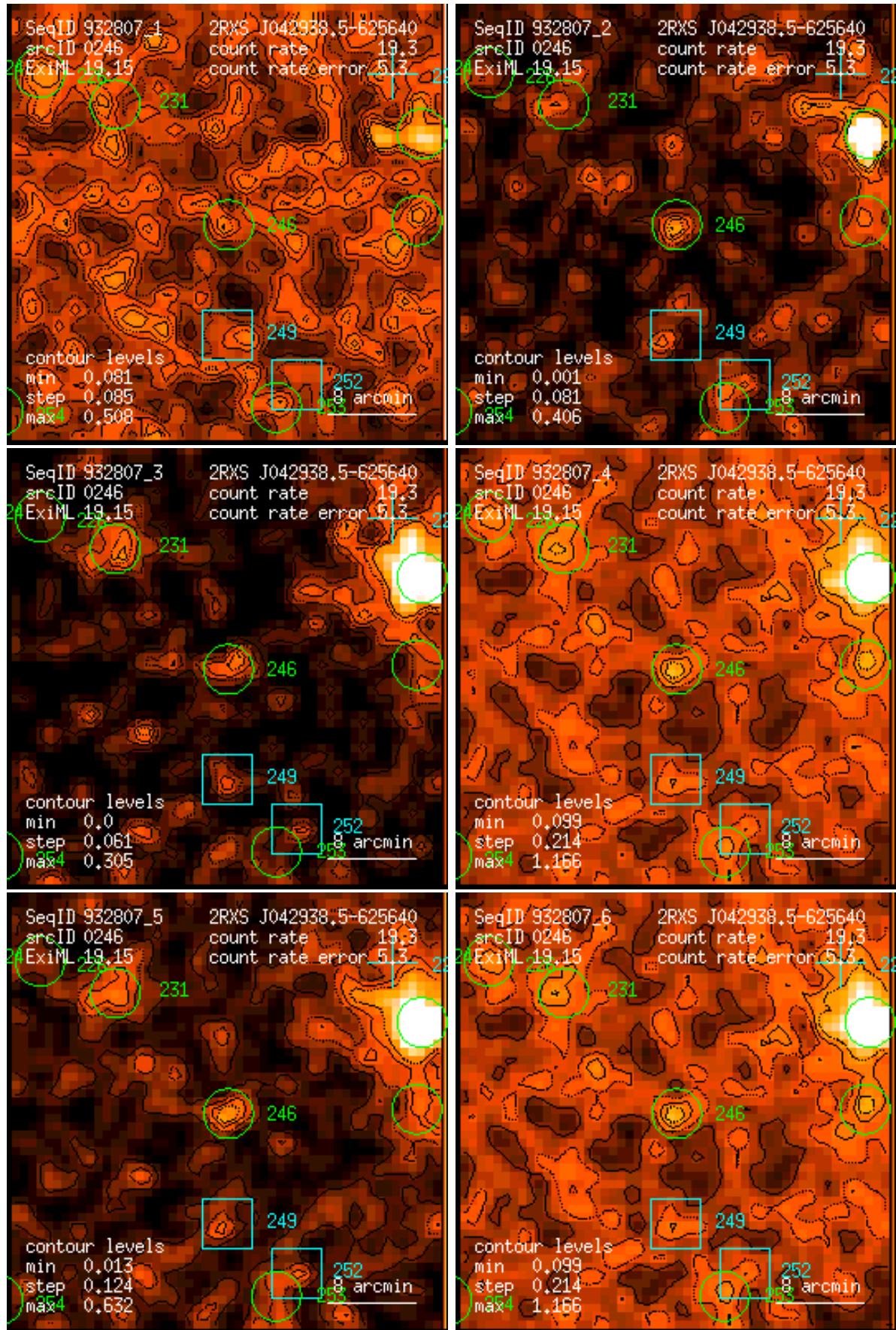
Figure 246: RASS 932807: detection 0246: band rate images, Gaussian filter: (1) PSPC channels 11 – 41, (2) 52 – 90, (3) 91 – 201, (4) 11 – 235, (5) 52 – 201, (6) 11 – 201. Broad band rates in counts/ks. Band rate contour levels in counts/ks/arcmin 2 .
