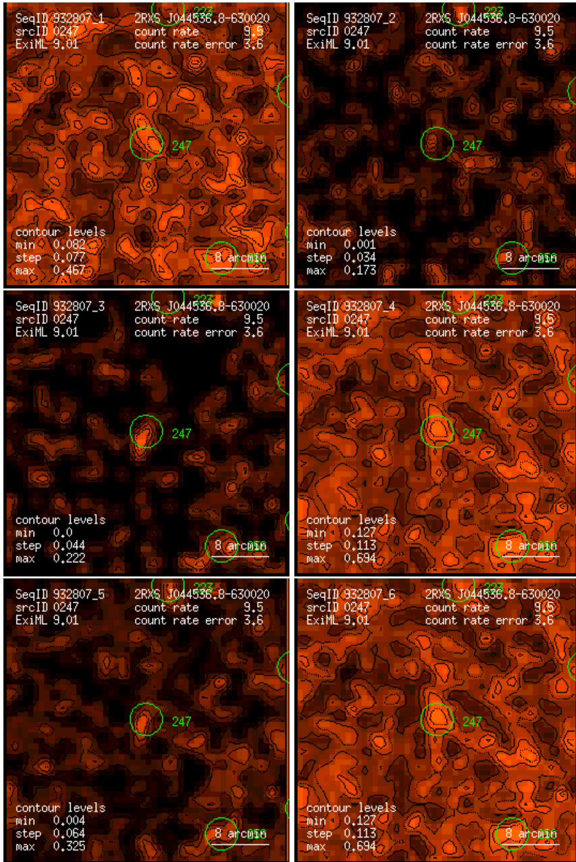
Figure 247: RASS 932807: detection 0247: band rate images, Gaussian filter: (1) PSPC channels 11 – 41, (2) 52 – 90, (3) 91 – 201, (4) 11 – 235, (5) 52 – 201, (6) 11 – 201. Broad band rates in counts/ks. Band rate contour levels in counts/ks/arcmin 2 .
