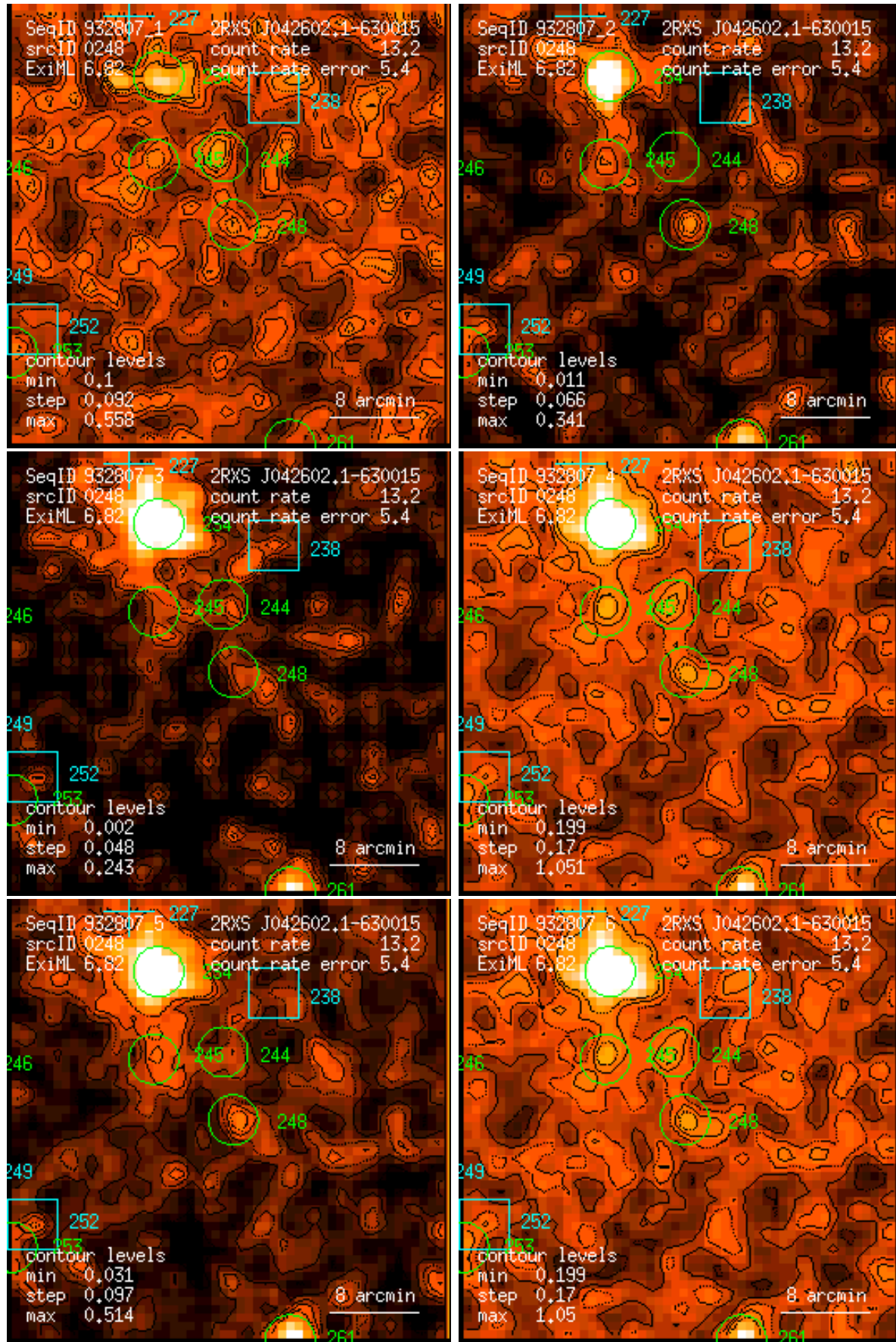
Figure 248: RASS 932807: detection 0248: band rate images, Gaussian filter: (1) PSPC channels 11 – 41, (2) 52 – 90, (3) 91 – 201, (4) 11 – 235, (5) 52 – 201, (6) 11 – 201. Broad band rates in counts/ks. Band rate contour levels in counts/ks/arcmin 2 .
