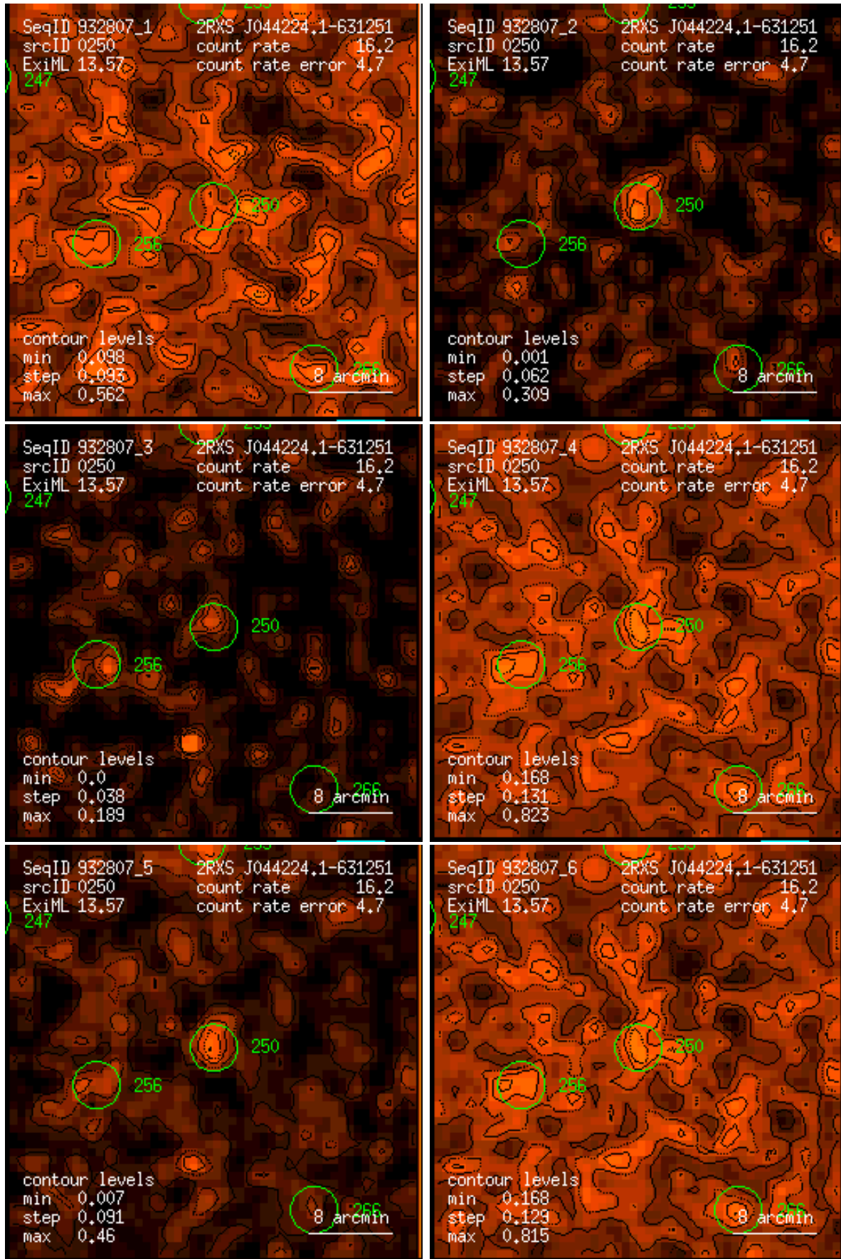
Figure 250: RASS 932807: detection 0250: band rate images, Gaussian filter: (1) PSPC channels 11 – 41, (2) 52 – 90, (3) 91 – 201, (4) 11 – 235, (5) 52 – 201, (6) 11 – 201. Broad band rates in counts/ks. Band rate contour levels in counts/ks/arcmin 2 .
