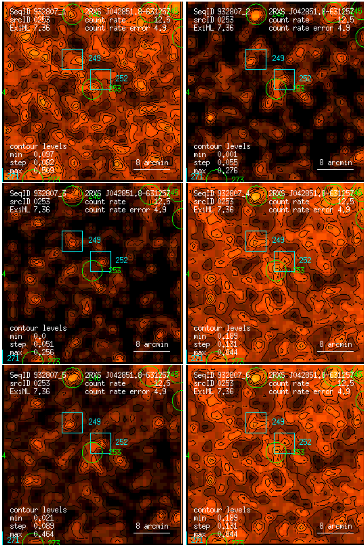
Figure 253: RASS 932807: detection 0253: band rate images, Gaussian filter: (1) PSPC channels 11 – 41, (2) 52 – 90, (3) 91 – 201, (4) 11 – 235, (5) 52 – 201, (6) 11 – 201. Broad band rates in counts/ks. Band rate contour levels in counts/ks/arcmin 2 .
