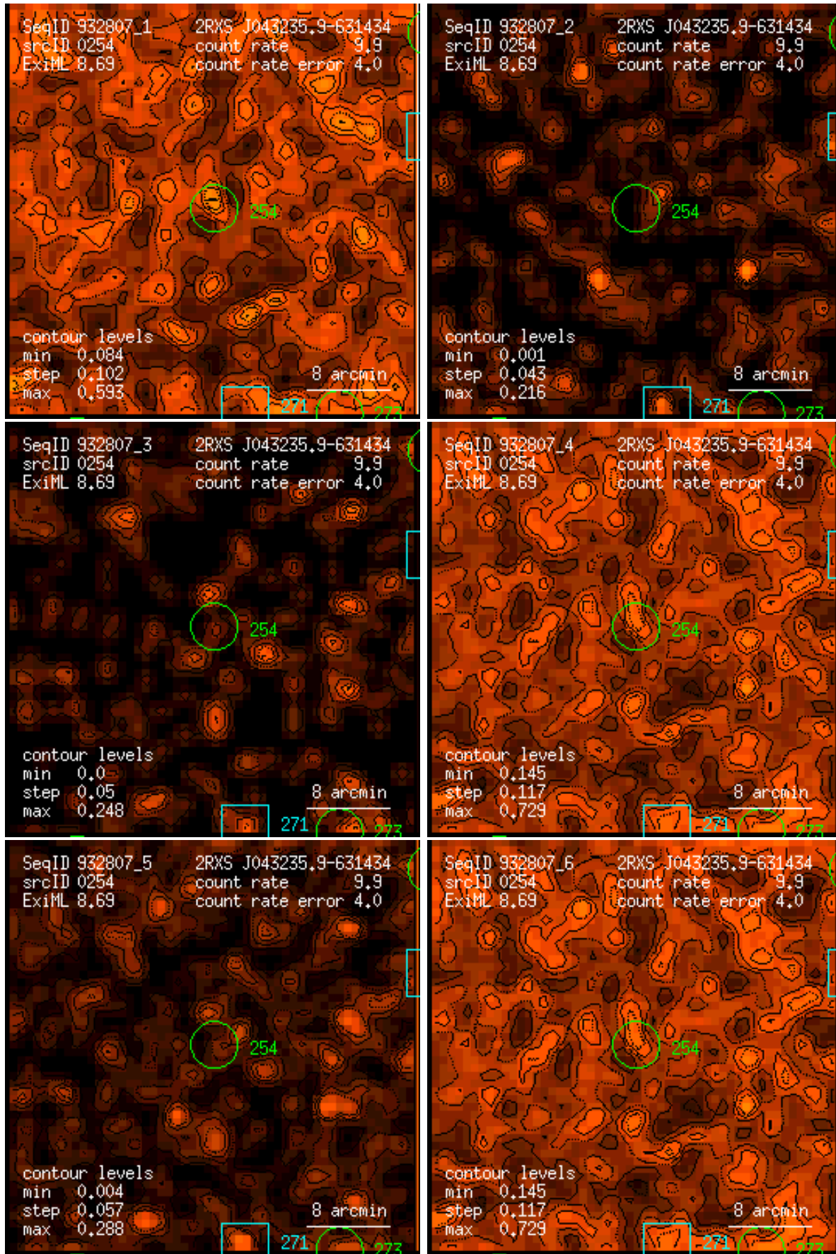
Figure 254: RASS 932807: detection 0254: band rate images, Gaussian filter: (1) PSPC channels 11 – 41, (2) 52 – 90, (3) 91 – 201, (4) 11 – 235, (5) 52 – 201, (6) 11 – 201. Broad band rates in counts/ks. Band rate contour levels in counts/ks/arcmin 2 .
