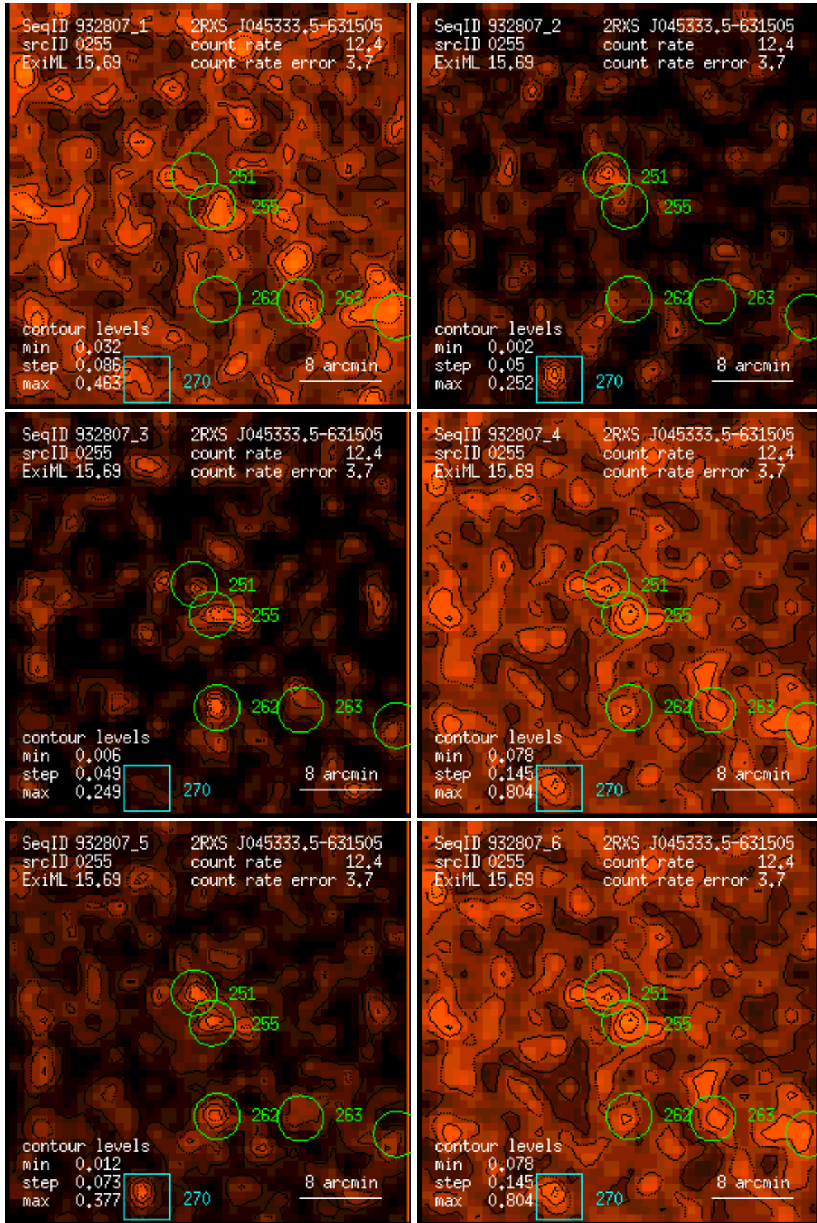
Figure 255: RASS 932807: detection 0255: band rate images, Gaussian filter: (1) PSPC channels 11 – 41, (2) 52 – 90, (3) 91 – 201, (4) 11 – 235, (5) 52 – 201, (6) 11 – 201. Broad band rates in counts/ks. Band rate contour levels in counts/ks/arcmin 2 .
