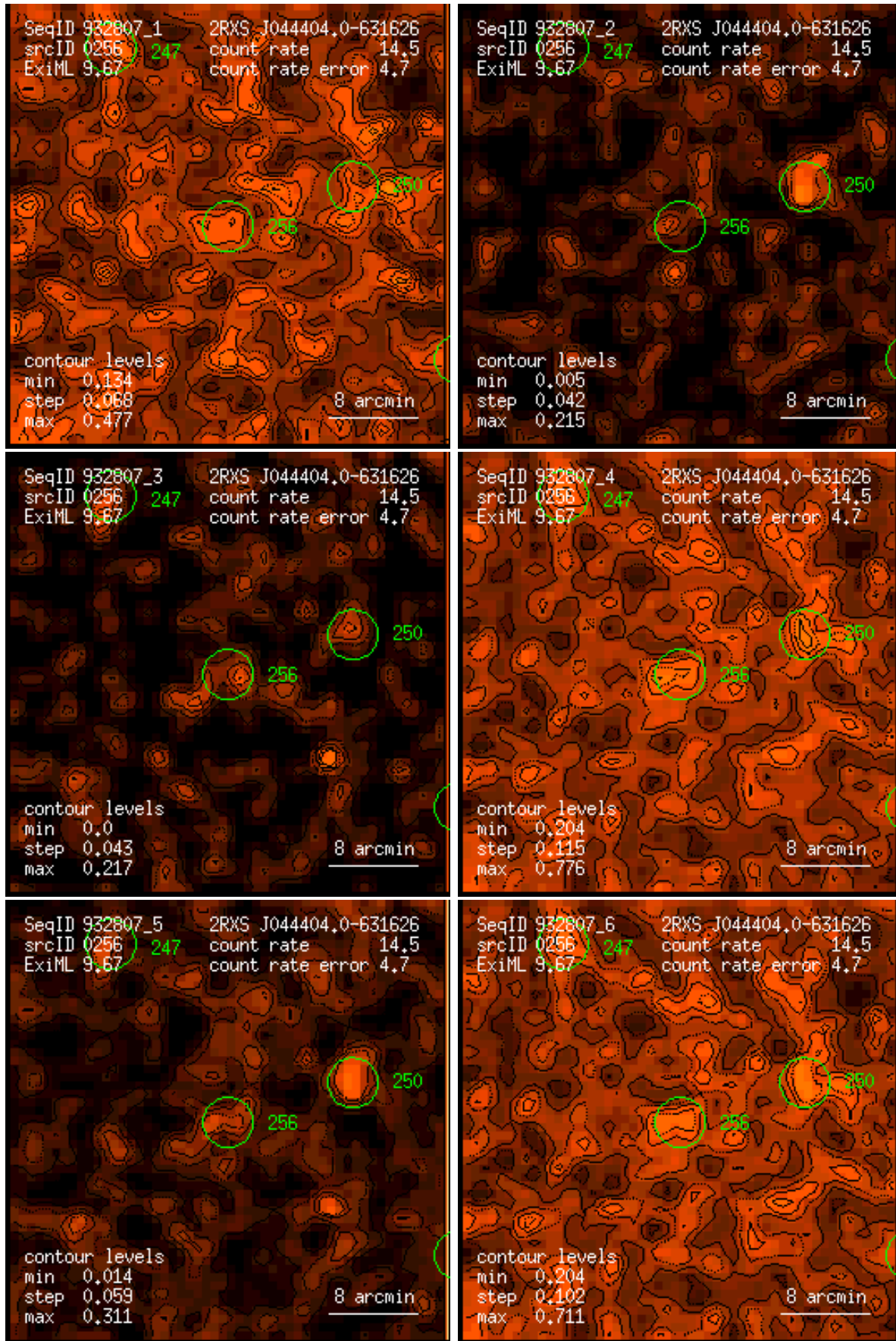
Figure 256: RASS 932807: detection 0256: band rate images, Gaussian filter: (1) PSPC channels 11 – 41, (2) 52 – 90, (3) 91 – 201, (4) 11 – 235, (5) 52 – 201, (6) 11 – 201. Broad band rates in counts/ks. Band rate contour levels in counts/ks/arcmin 2 .
