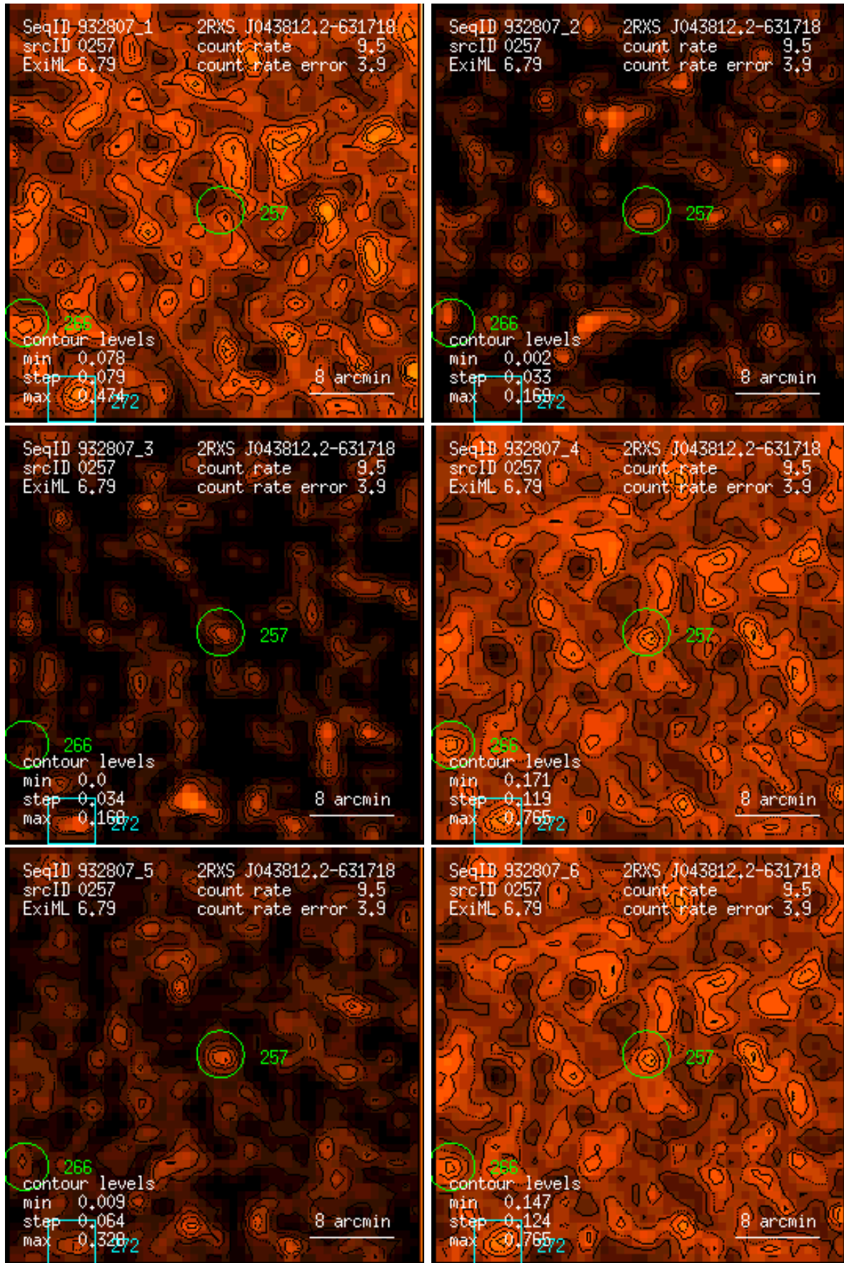
Figure 257: RASS 932807: detection 0257: band rate images, Gaussian filter: (1) PSPC channels 11 – 41, (2) 52 – 90, (3) 91 – 201, (4) 11 – 235, (5) 52 – 201, (6) 11 – 201. Broad band rates in counts/ks. Band rate contour levels in counts/ks/arcmin 2 .
