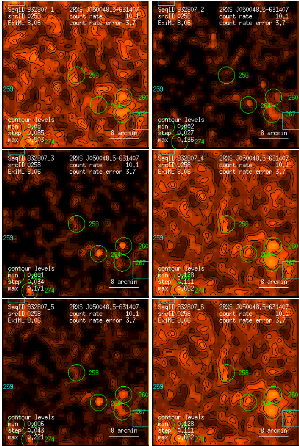
Figure 258: RASS 932807: detection 0258: band rate images, Gaussian filter: (1) PSPC channels 11 – 41, (2) 52 – 90, (3) 91 – 201, (4) 11 – 235, (5) 52 – 201, (6) 11 – 201. Broad band rates in counts/ks. Band rate contour levels in counts/ks/arcmin 2 .
