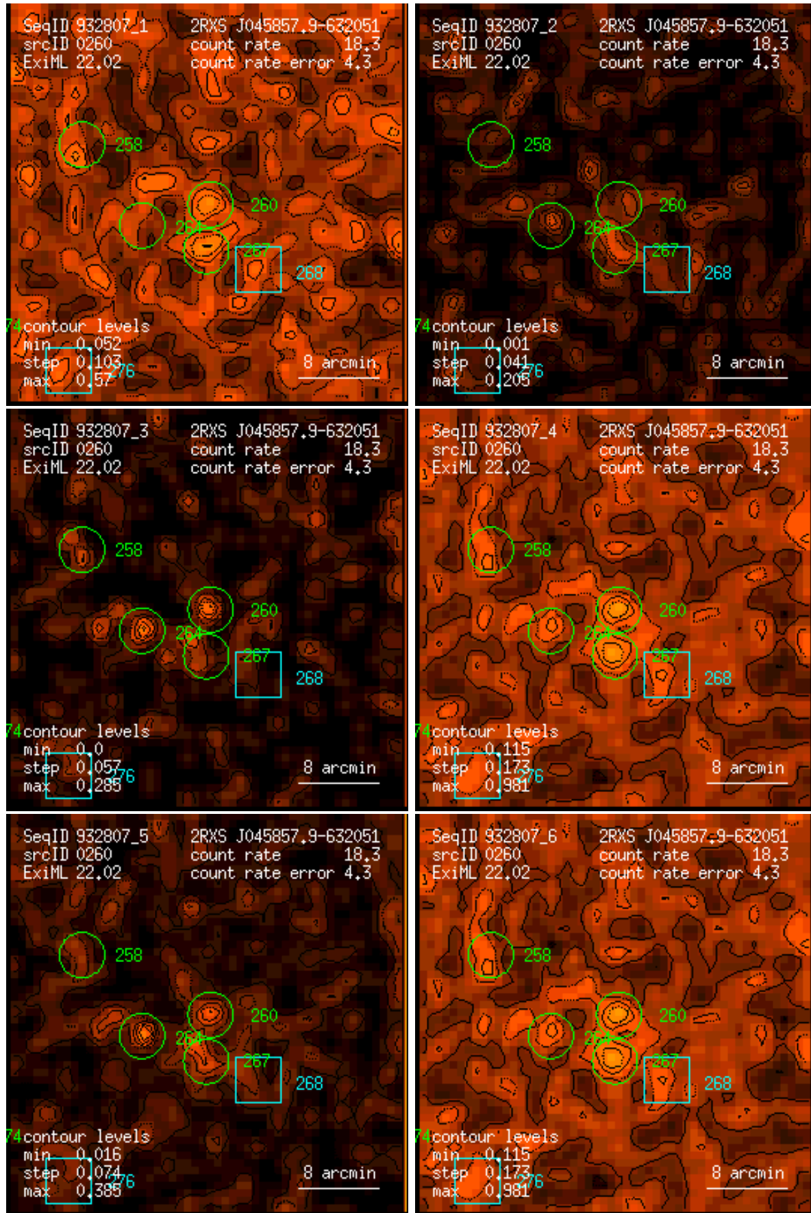
Figure 260: RASS 932807: detection 0260: band rate images, Gaussian filter: (1) PSPC channels 11 – 41, (2) 52 – 90, (3) 91 – 201, (4) 11 – 235, (5) 52 – 201, (6) 11 – 201. Broad band rates in counts/ks. Band rate contour levels in counts/ks/arcmin 2 .
