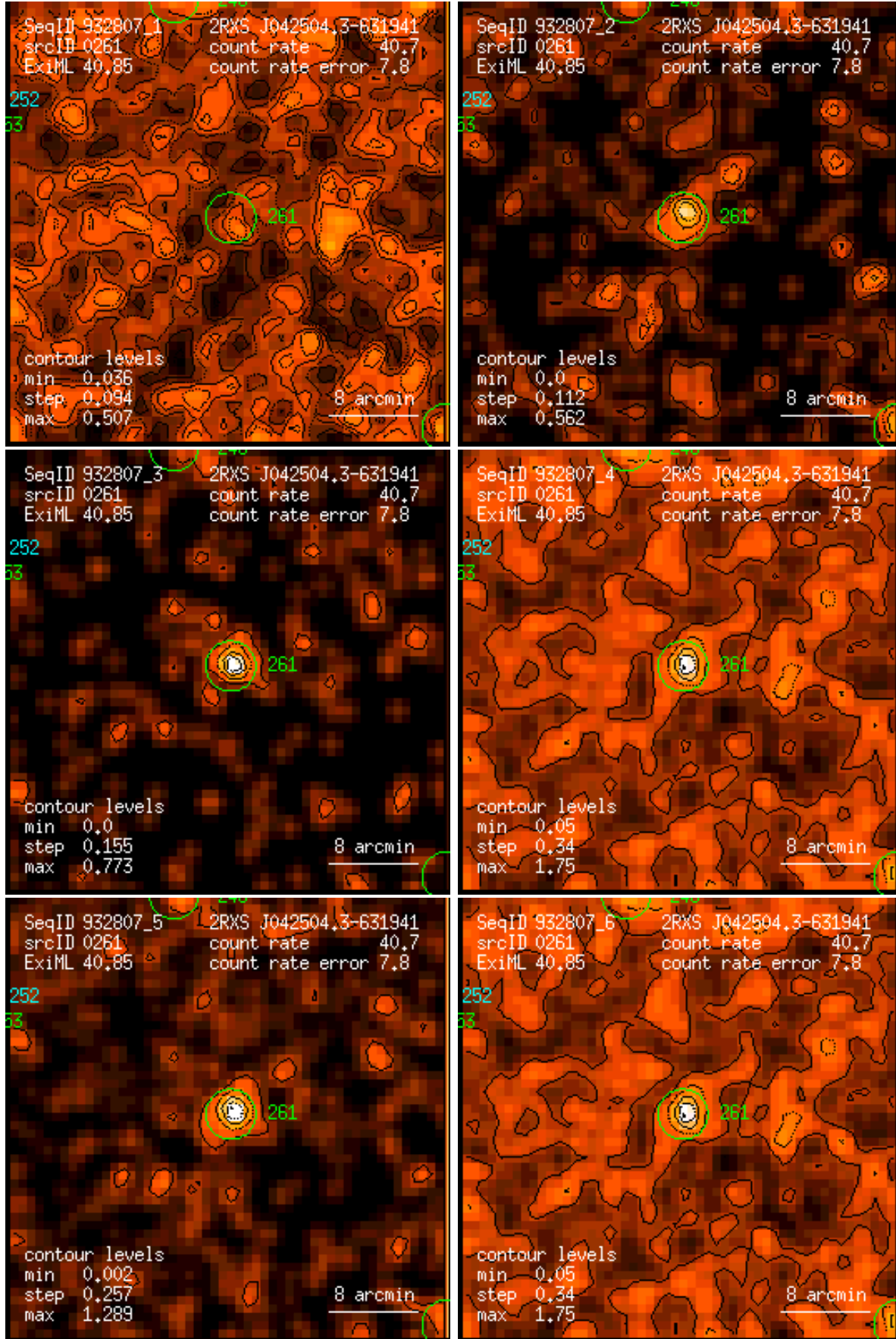
Figure 261: RASS 932807: detection 0261: band rate images, Gaussian filter: (1) PSPC channels 11 – 41, (2) 52 – 90, (3) 91 – 201, (4) 11 – 235, (5) 52 – 201, (6) 11 – 201. Broad band rates in counts/ks. Band rate contour levels in counts/ks/arcmin 2 .
