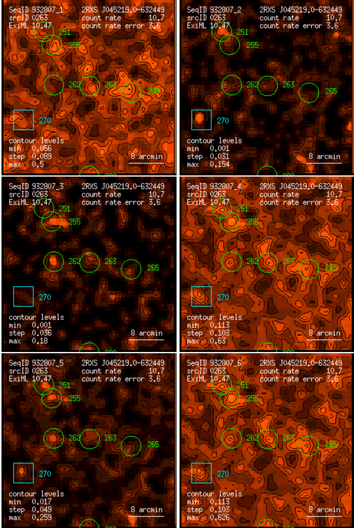
Figure 263: RASS 932807: detection 0263: band rate images, Gaussian filter: (1) PSPC channels 11 – 41, (2) 52 – 90, (3) 91 – 201, (4) 11 – 235, (5) 52 – 201, (6) 11 – 201. Broad band rates in counts/ks. Band rate contour levels in counts/ks/arcmin 2 .
