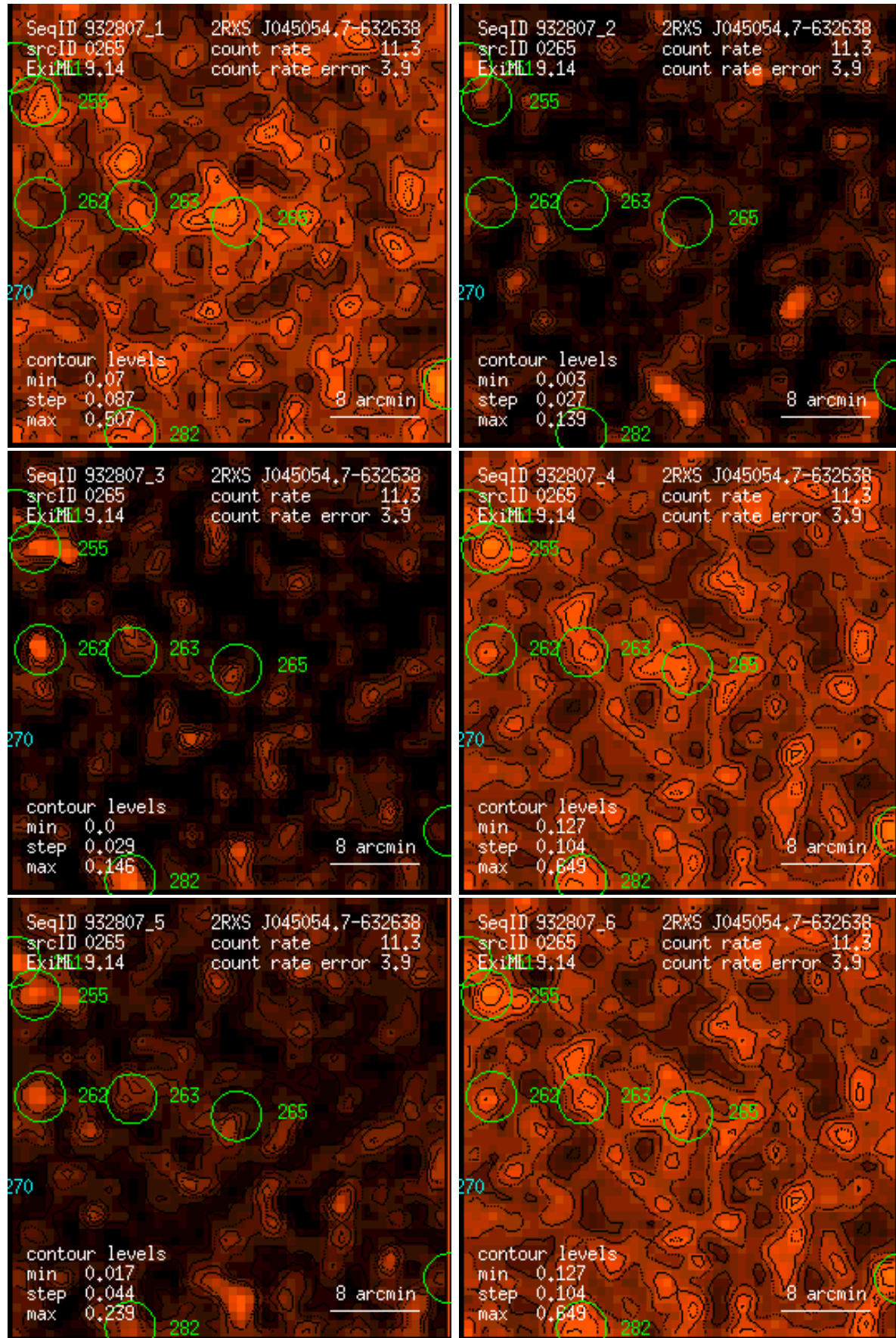
Figure 265: RASS 932807: detection 0265: band rate images, Gaussian filter: (1) PSPC channels 11 – 41, (2) 52 – 90, (3) 91 – 201, (4) 11 – 235, (5) 52 – 201, (6) 11 – 201. Broad band rates in counts/ks. Band rate contour levels in counts/ks/arcmin 2 .
