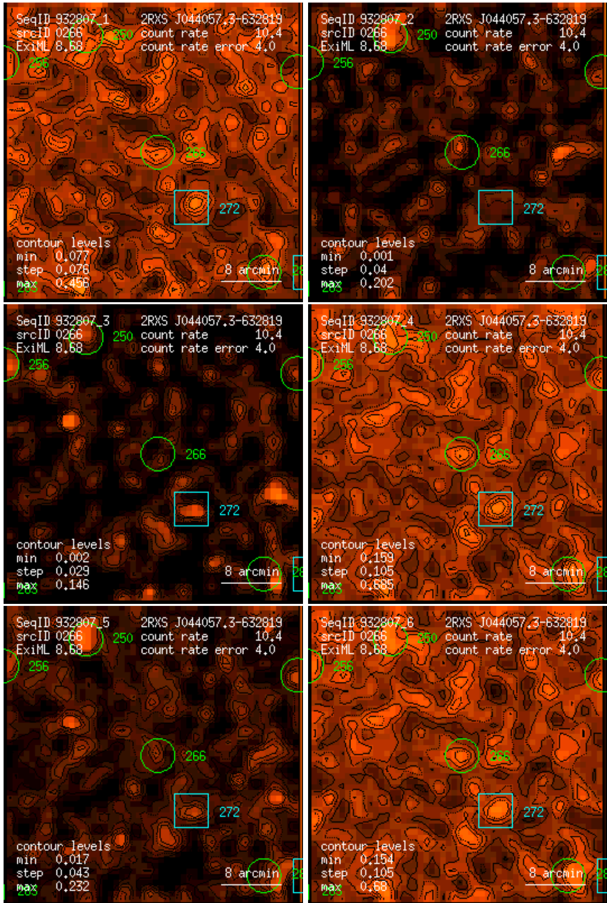
Figure 266: RASS 932807: detection 0266: band rate images, Gaussian filter: (1) PSPC channels 11 – 41, (2) 52 – 90, (3) 91 – 201, (4) 11 – 235, (5) 52 – 201, (6) 11 – 201. Broad band rates in counts/ks. Band rate contour levels in counts/ks/arcmin 2 .
