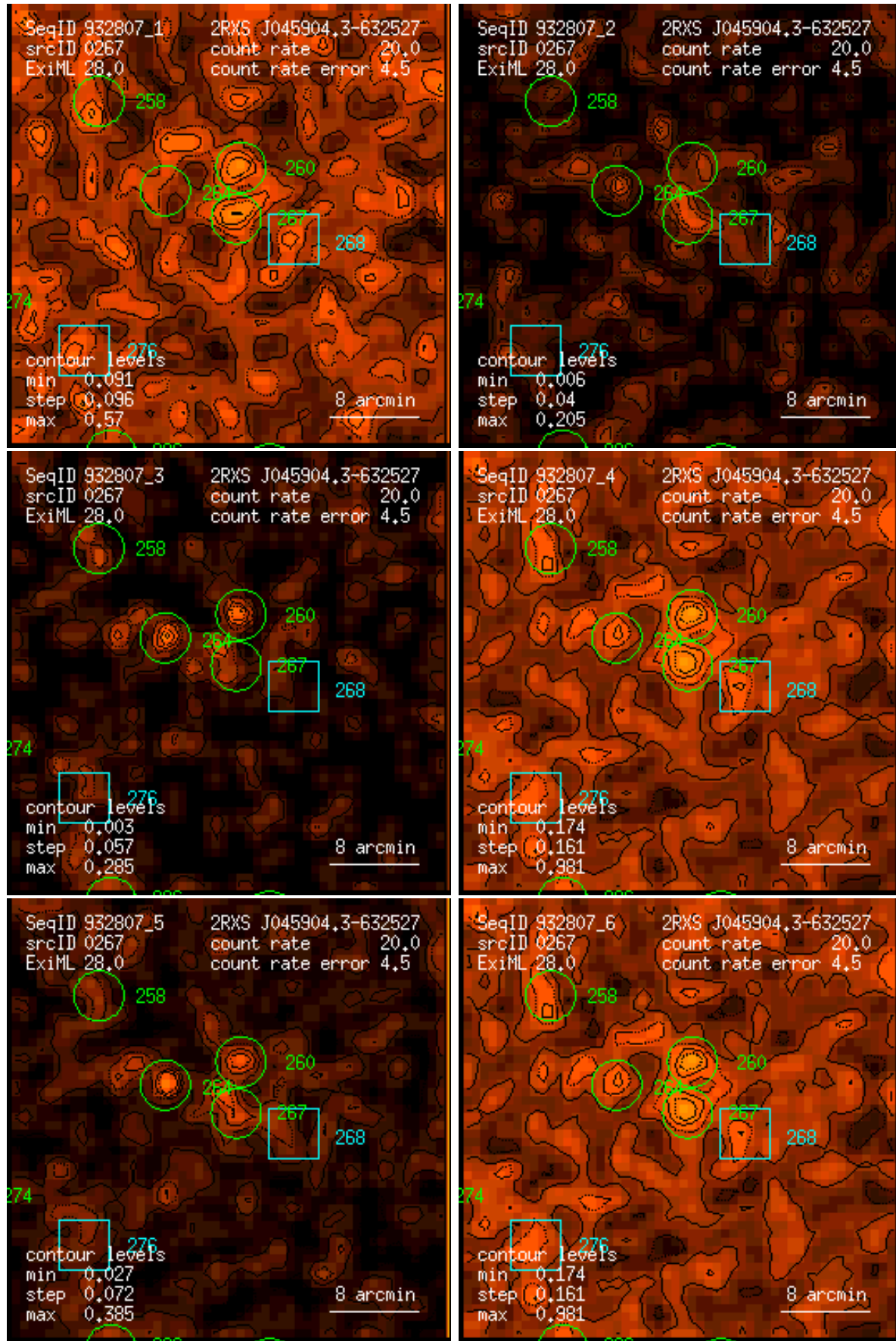
Figure 267: RASS 932807: detection 0267: band rate images, Gaussian filter: (1) PSPC channels 11 – 41, (2) 52 – 90, (3) 91 – 201, (4) 11 – 235, (5) 52 – 201, (6) 11 – 201. Broad band rates in counts/ks. Band rate contour levels in counts/ks/arcmin 2 .
