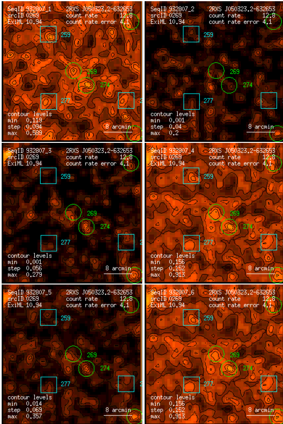
Figure 269: RASS 932807: detection 0269: band rate images, Gaussian filter: (1) PSPC channels 11 – 41, (2) 52 – 90, (3) 91 – 201, (4) 11 – 235, (5) 52 – 201, (6) 11 – 201. Broad band rates in counts/ks. Band rate contour levels in counts/ks/arcmin 2 .
