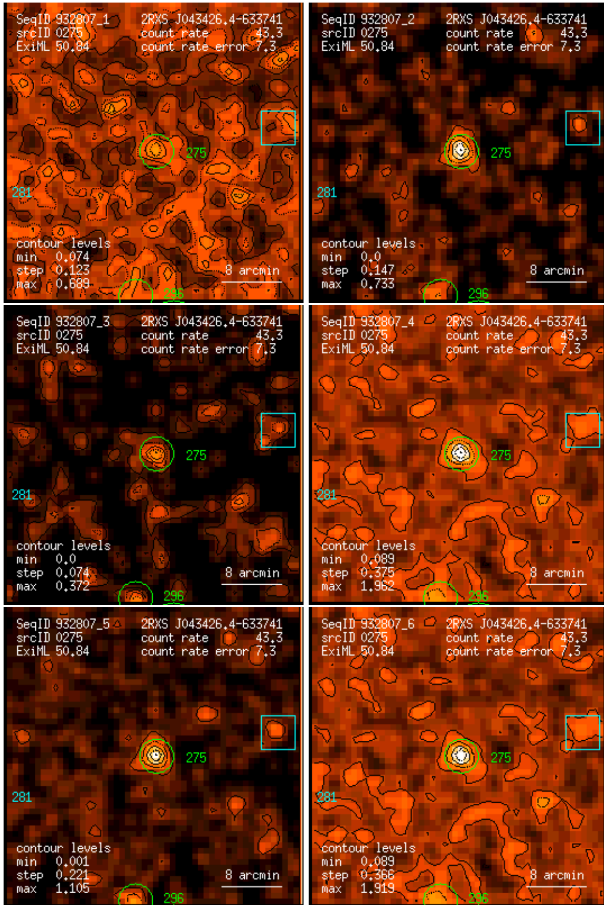
Figure 275: RASS 932807: detection 0275: band rate images, Gaussian filter: (1) PSPC channels 11 – 41, (2) 52 – 90, (3) 91 – 201, (4) 11 – 235, (5) 52 – 201, (6) 11 – 201. Broad band rates in counts/ks. Band rate contour levels in counts/ks/arcmin 2 .
