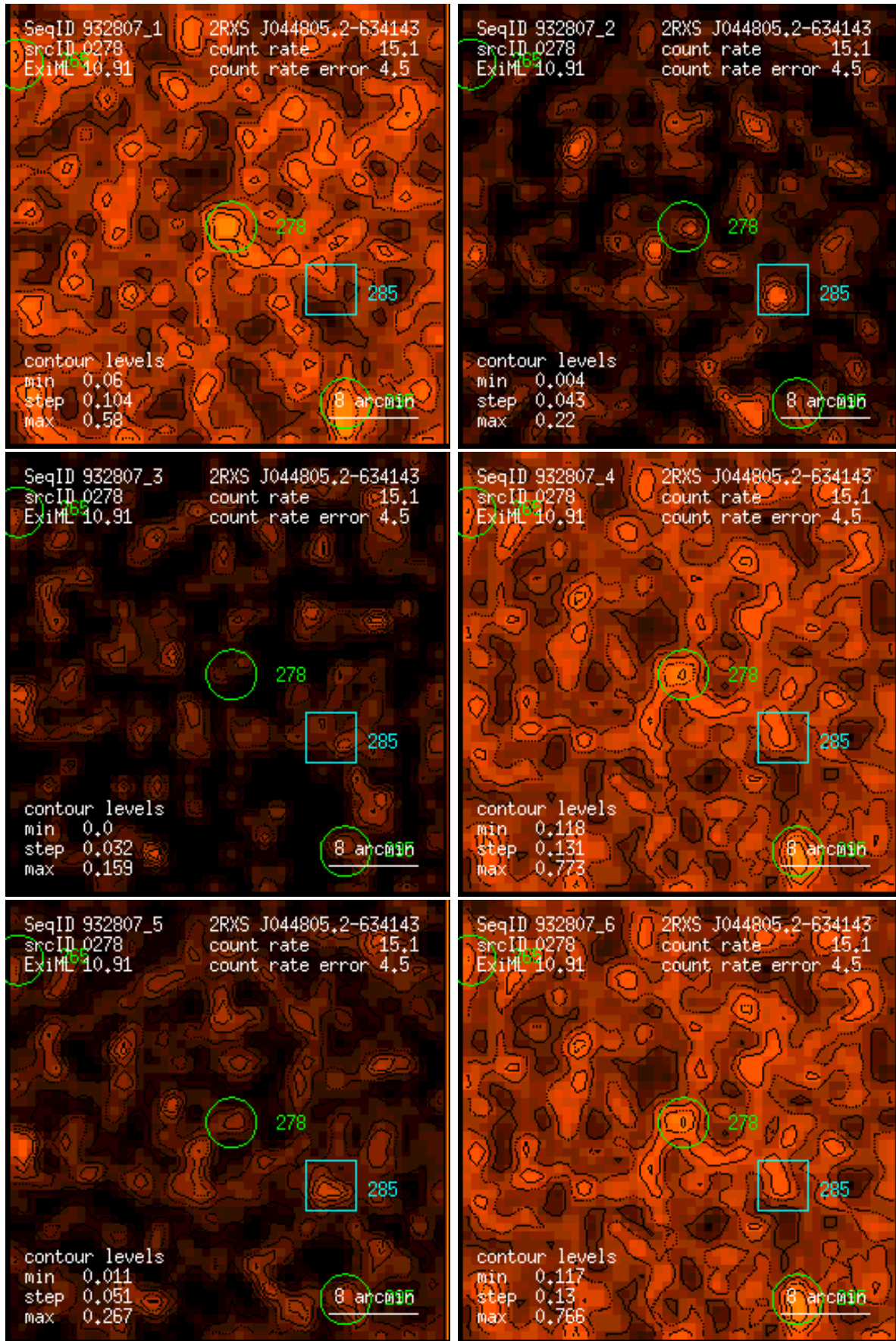
Figure 278: RASS 932807: detection 0278: band rate images, Gaussian filter: (1) PSPC channels 11 – 41, (2) 52 – 90, (3) 91 – 201, (4) 11 – 235, (5) 52 – 201, (6) 11 – 201. Broad band rates in counts/ks. Band rate contour levels in counts/ks/arcmin 2 .
