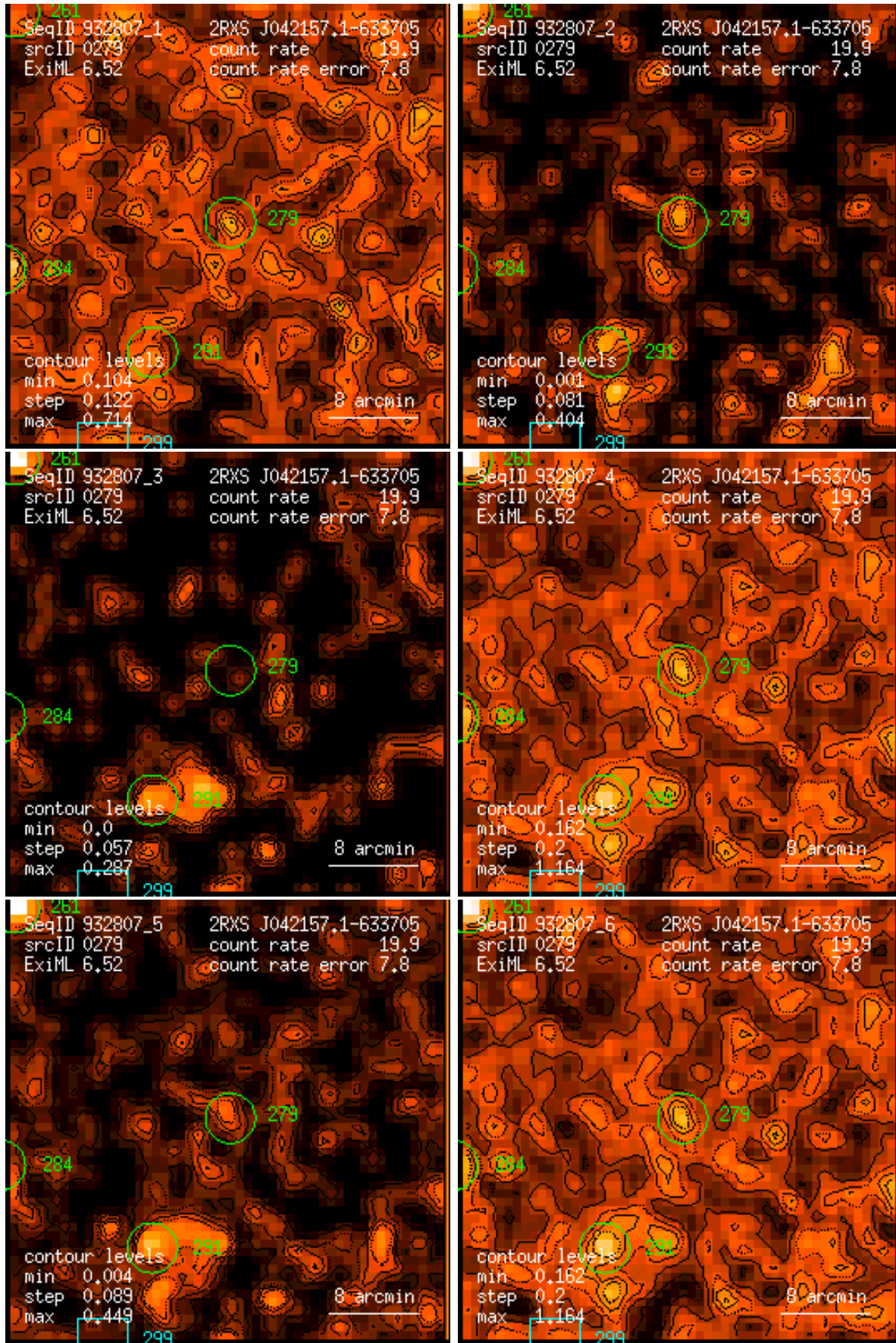
Figure 279: RASS 932807: detection 0279: band rate images, Gaussian filter: (1) PSPC channels 11 – 41, (2) 52 – 90, (3) 91 – 201, (4) 11 – 235, (5) 52 – 201, (6) 11 – 201. Broad band rates in counts/ks. Band rate contour levels in counts/ks/arcmin 2 .
