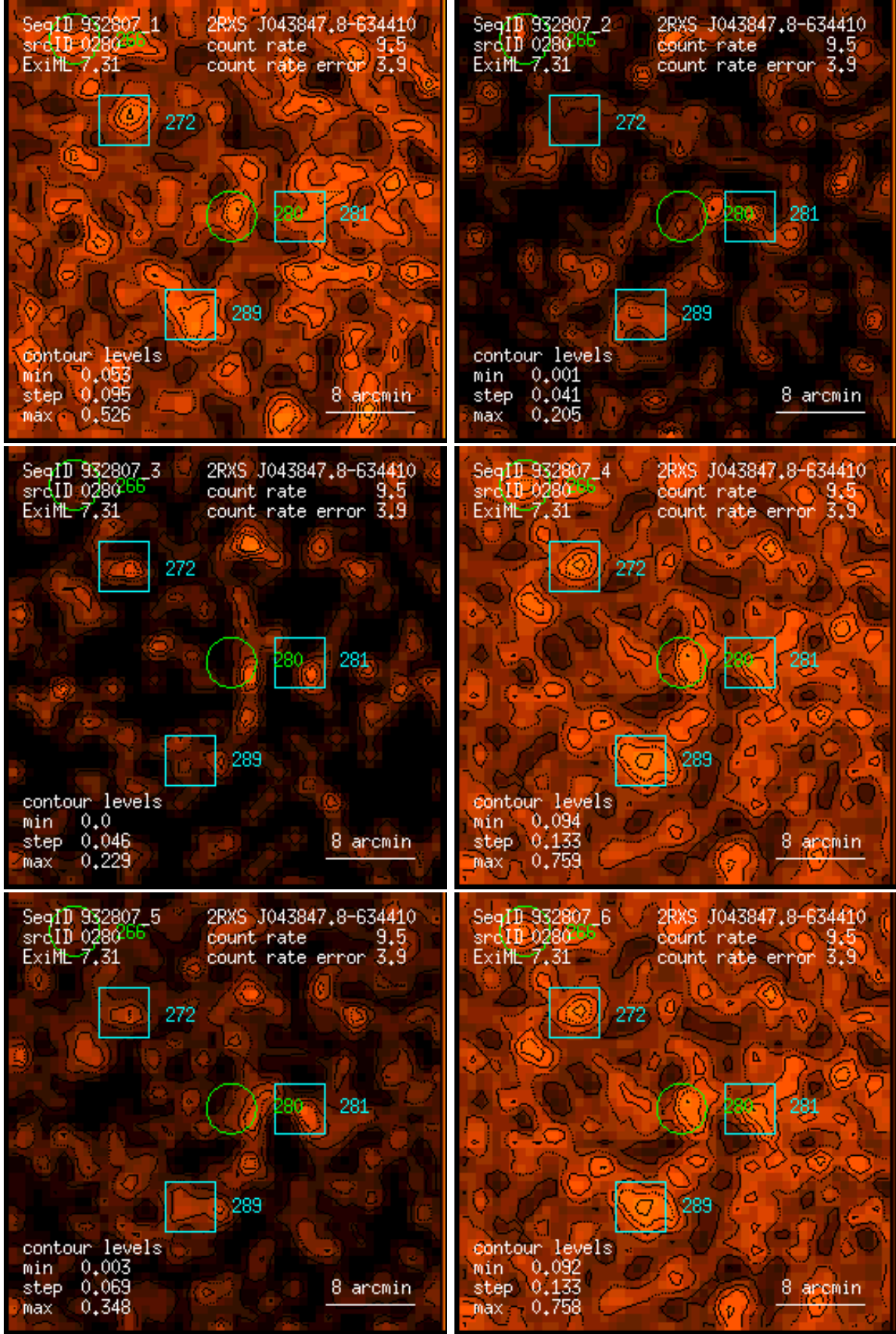
Figure 280: RASS 932807: detection 0280: band rate images, Gaussian filter: (1) PSPC channels 11 – 41, (2) 52 – 90, (3) 91 – 201, (4) 11 – 235, (5) 52 – 201, (6) 11 – 201. Broad band rates in counts/ks. Band rate contour levels in counts/ks/arcmin 2 .
