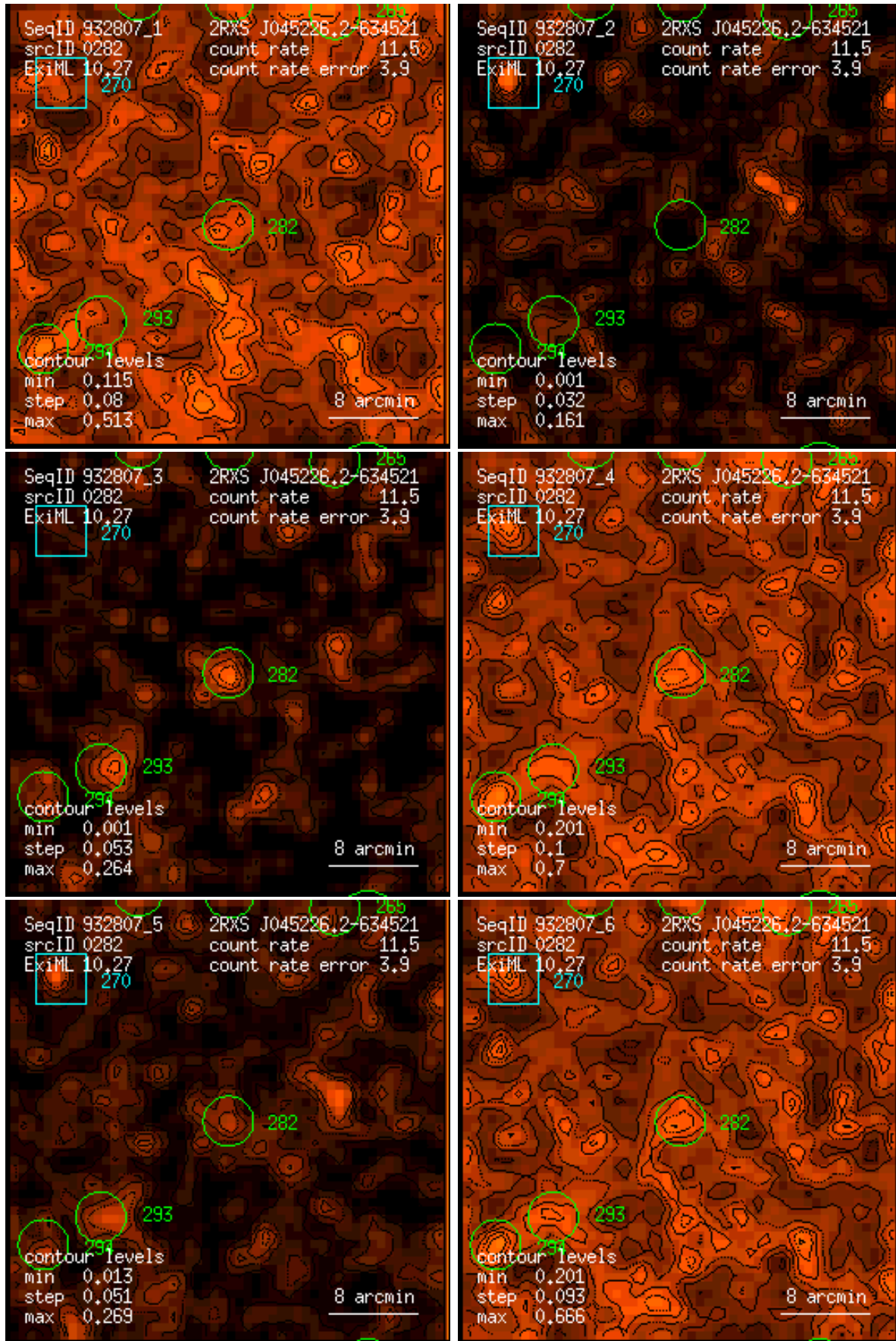
Figure 282: RASS 932807: detection 0282: band rate images, Gaussian filter: (1) PSPC channels 11 – 41, (2) 52 – 90, (3) 91 – 201, (4) 11 – 235, (5) 52 – 201, (6) 11 – 201. Broad band rates in counts/ks. Band rate contour levels in counts/ks/arcmin 2 .
