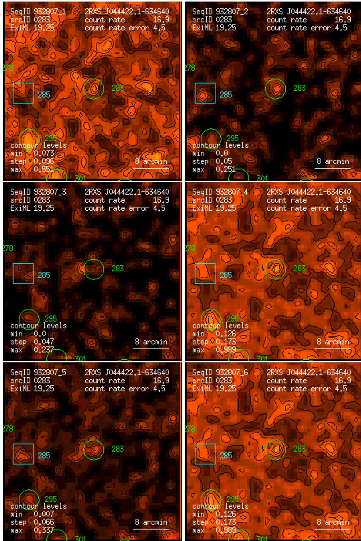
Figure 283: RASS 932807: detection 0283: band rate images, Gaussian filter: (1) PSPC channels 11 – 41, (2) 52 – 90, (3) 91 – 201, (4) 11 – 235, (5) 52 – 201, (6) 11 – 201. Broad band rates in counts/ks. Band rate contour levels in counts/ks/arcmin 2 .
