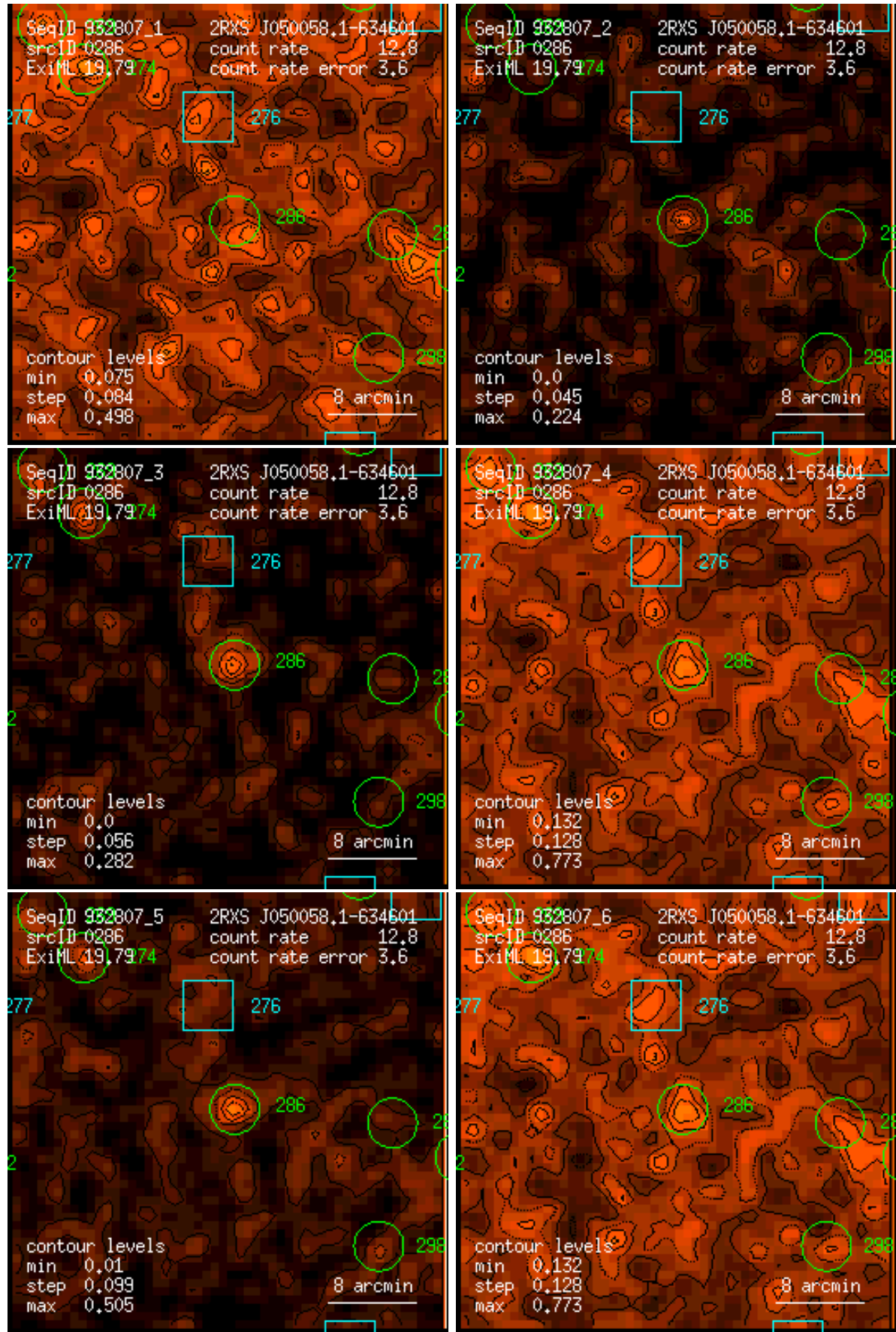
Figure 286: RASS 932807: detection 0286: band rate images, Gaussian filter: (1) PSPC channels 11 – 41, (2) 52 – 90, (3) 91 – 201, (4) 11 – 235, (5) 52 – 201, (6) 11 – 201. Broad band rates in counts/ks. Band rate contour levels in counts/ks/arcmin 2 .
