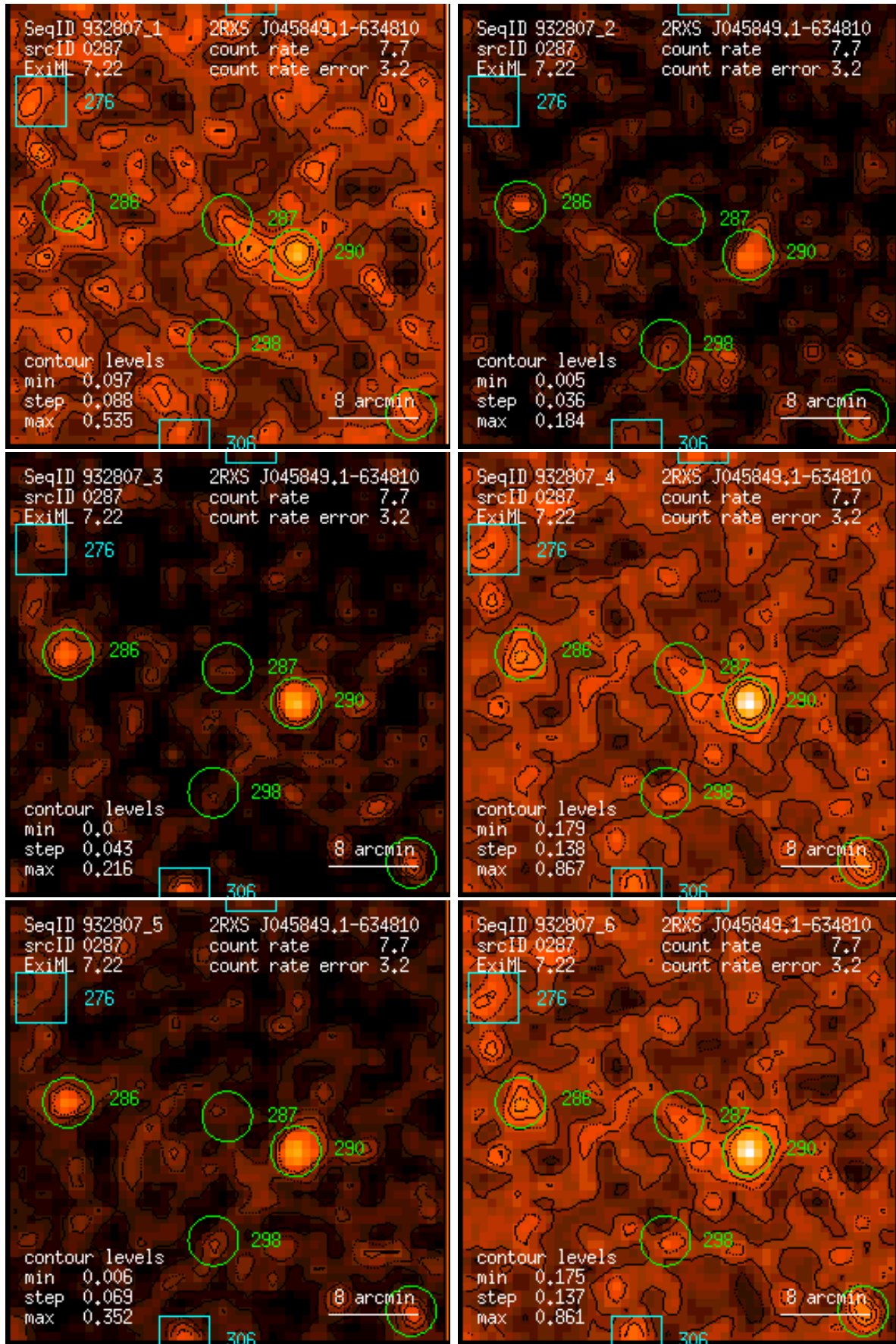
Figure 287: RASS 932807: detection 0287: band rate images, Gaussian filter: (1) PSPC channels 11 – 41, (2) 52 – 90, (3) 91 – 201, (4) 11 – 235, (5) 52 – 201, (6) 11 – 201. Broad band rates in counts/ks. Band rate contour levels in counts/ks/arcmin 2 .
