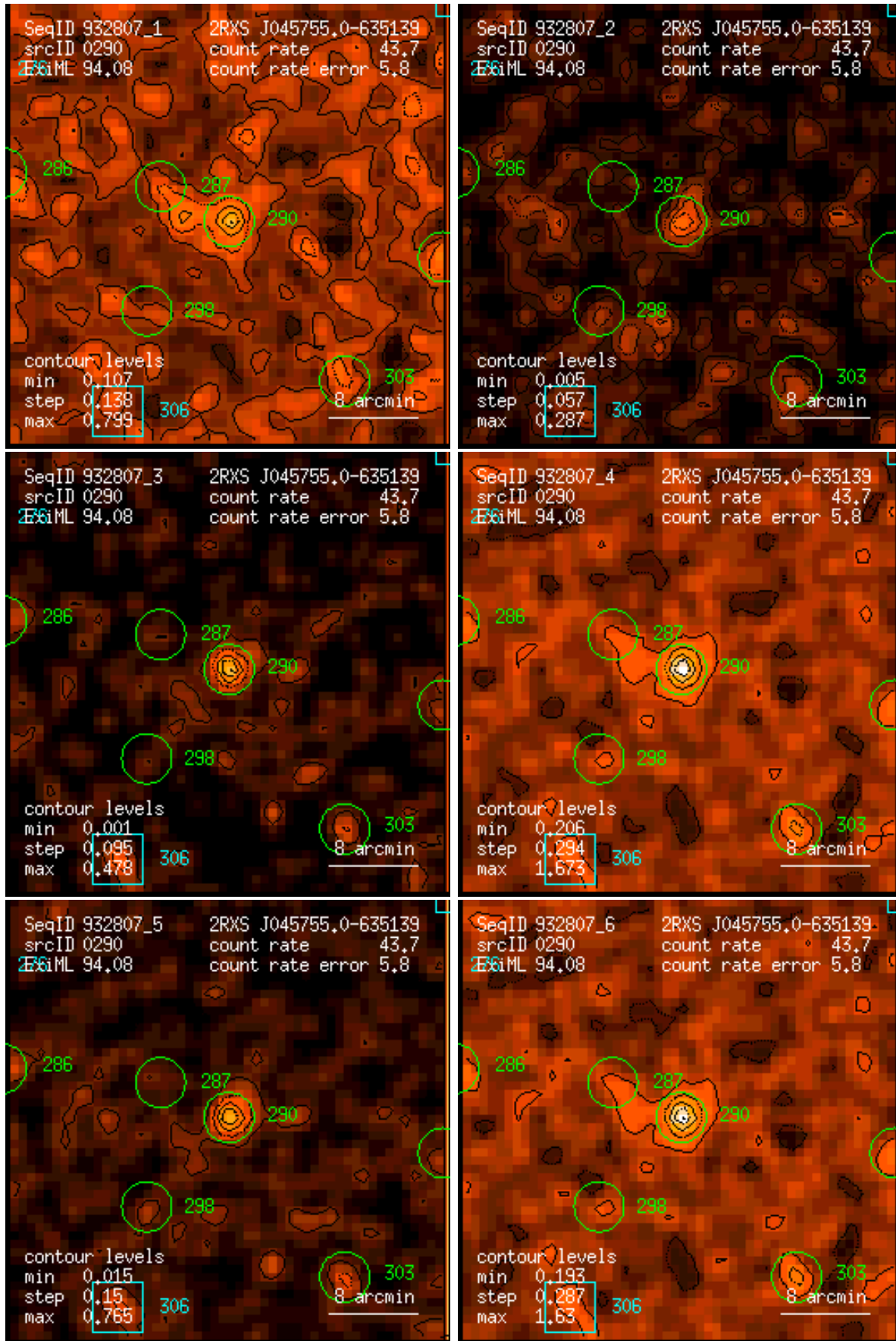
Figure 290: RASS 932807: detection 0290: band rate images, Gaussian filter: (1) PSPC channels 11 – 41, (2) 52 – 90, (3) 91 – 201, (4) 11 – 235, (5) 52 – 201, (6) 11 – 201. Broad band rates in counts/ks. Band rate contour levels in counts/ks/arcmin 2 .
