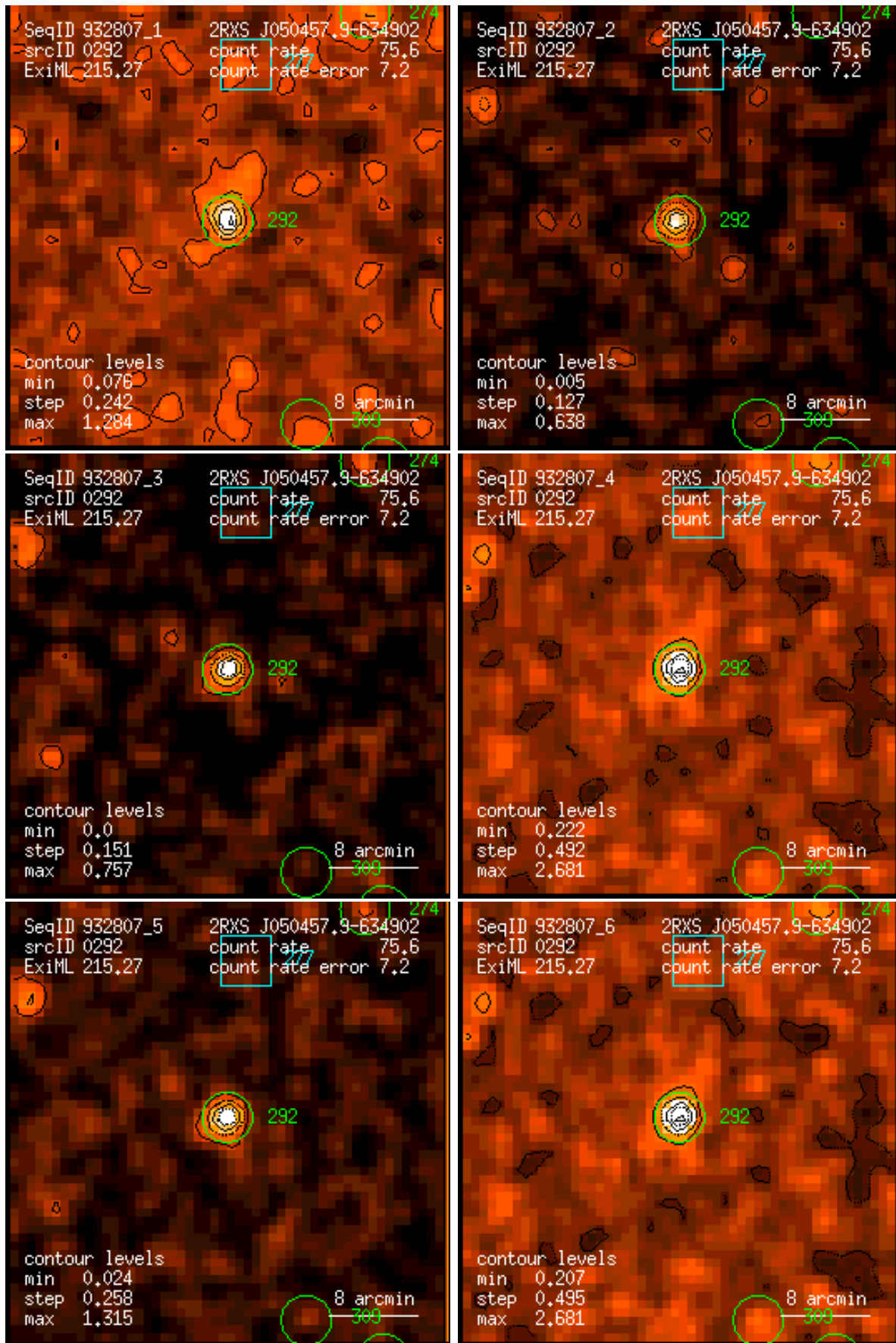
Figure 292: RASS 932807: detection 0292: band rate images, Gaussian filter: (1) PSPC channels 11 – 41, (2) 52 – 90, (3) 91 – 201, (4) 11 – 235, (5) 52 – 201, (6) 11 – 201. Broad band rates in counts/ks. Band rate contour levels in counts/ks/arcmin 2 .
