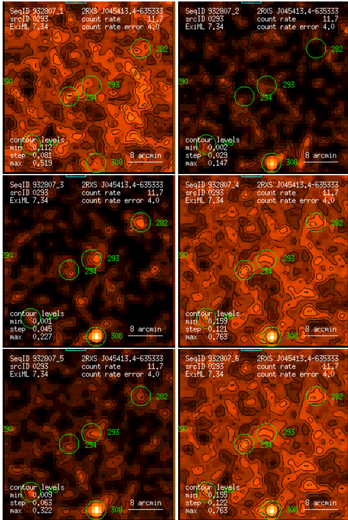
Figure 293: RASS 932807: detection 0293: band rate images, Gaussian filter: (1) PSPC channels 11 – 41, (2) 52 – 90, (3) 91 – 201, (4) 11 – 235, (5) 52 – 201, (6) 11 – 201. Broad band rates in counts/ks. Band rate contour levels in counts/ks/arcmin 2 .
