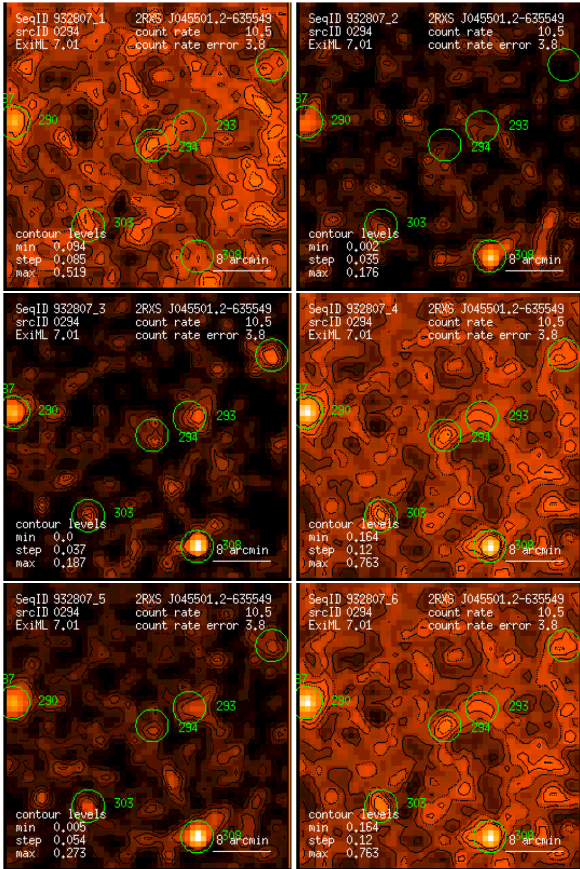
Figure 294: RASS 932807: detection 0294: band rate images, Gaussian filter: (1) PSPC channels 11 – 41, (2) 52 – 90, (3) 91 – 201, (4) 11 – 235, (5) 52 – 201, (6) 11 – 201. Broad band rates in counts/ks. Band rate contour levels in counts/ks/arcmin 2 .
