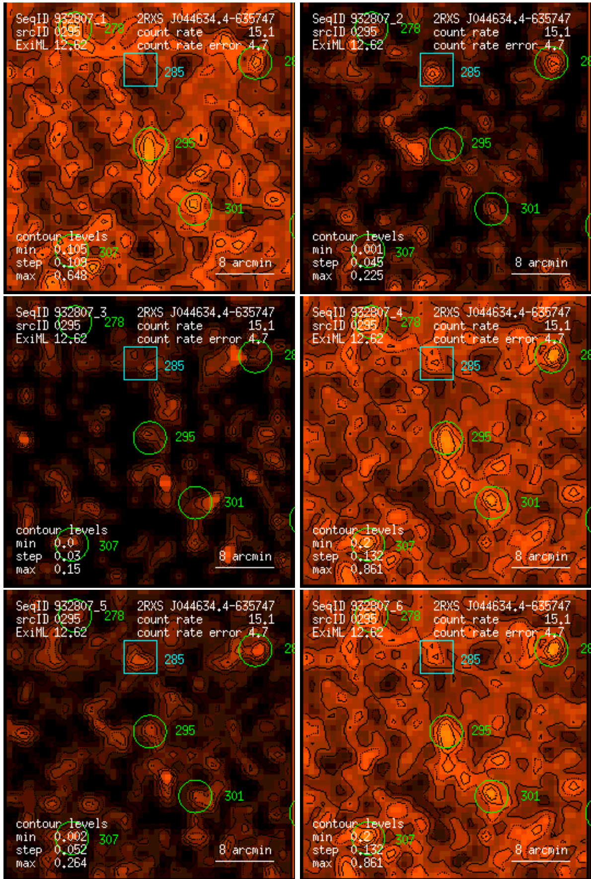
Figure 295: RASS 932807: detection 0295: band rate images, Gaussian filter: (1) PSPC channels 11 – 41, (2) 52 – 90, (3) 91 – 201, (4) 11 – 235, (5) 52 – 201, (6) 11 – 201. Broad band rates in counts/ks. Band rate contour levels in counts/ks/arcmin 2 .
