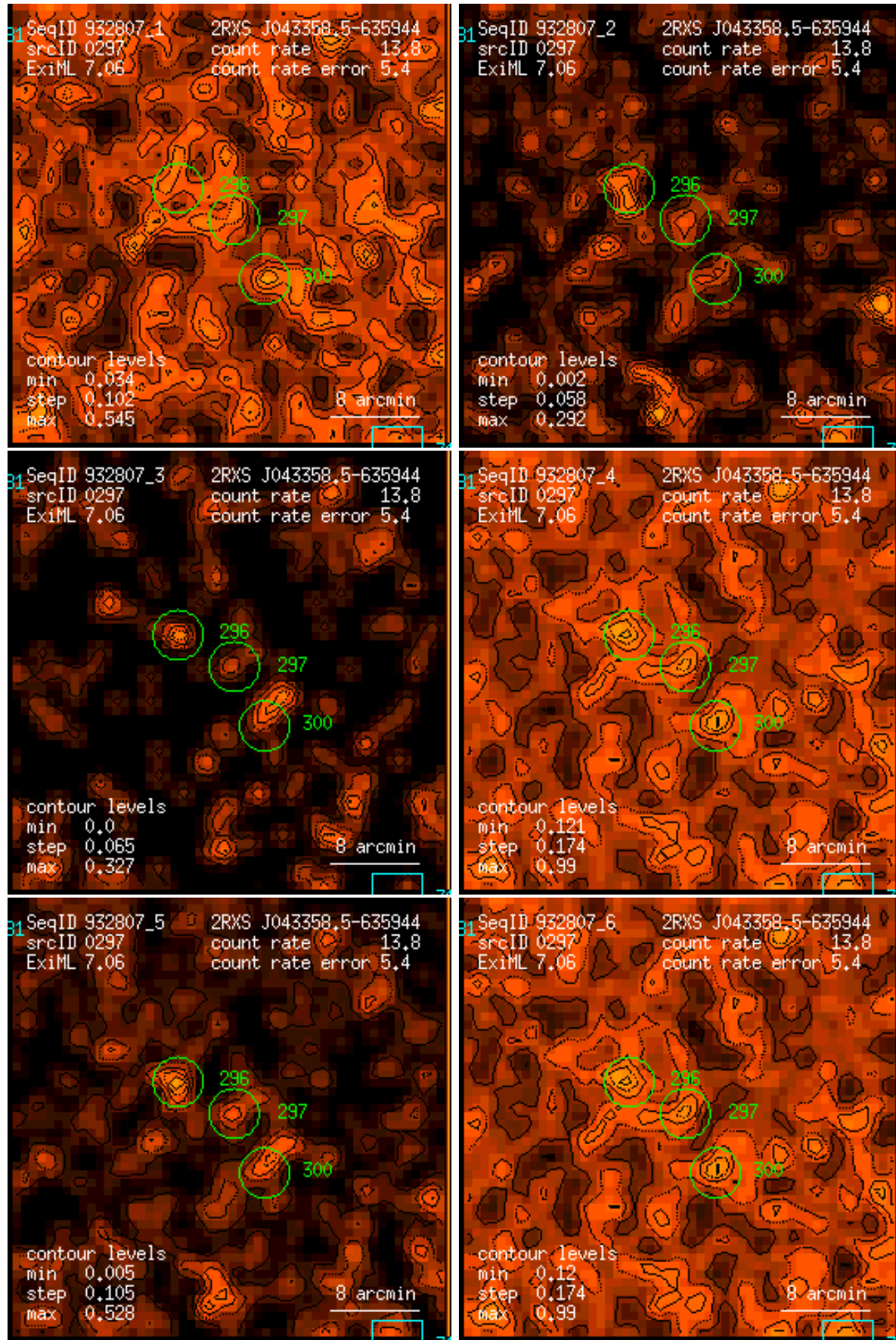
Figure 297: RASS 932807: detection 0297: band rate images, Gaussian filter: (1) PSPC channels 11 – 41, (2) 52 – 90, (3) 91 – 201, (4) 11 – 235, (5) 52 – 201, (6) 11 – 201. Broad band rates in counts/ks. Band rate contour levels in counts/ks/arcmin 2 .
