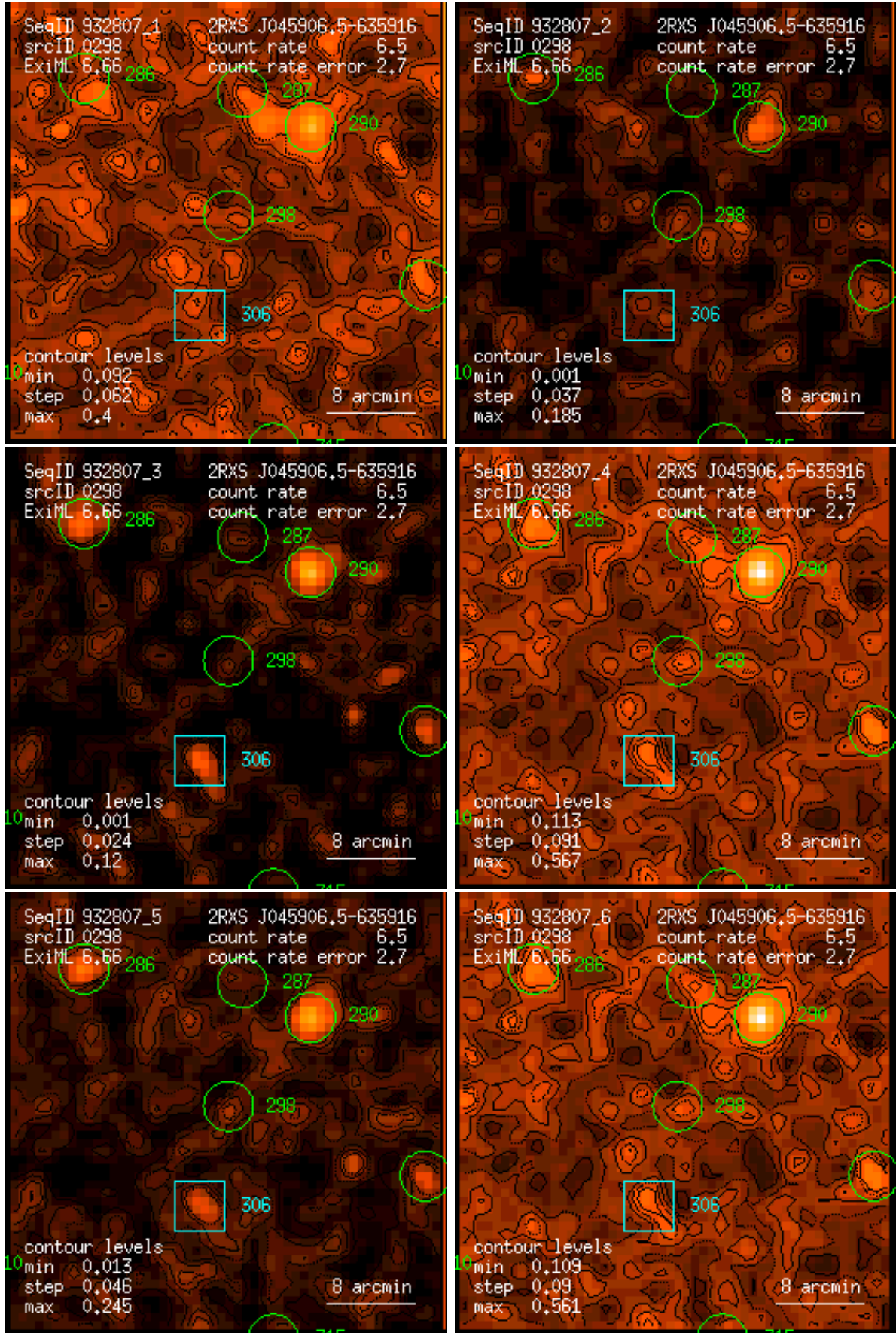
Figure 298: RASS 932807: detection 0298: band rate images, Gaussian filter: (1) PSPC channels 11 – 41, (2) 52 – 90, (3) 91 – 201, (4) 11 – 235, (5) 52 – 201, (6) 11 – 201. Broad band rates in counts/ks. Band rate contour levels in counts/ks/arcmin 2 .
