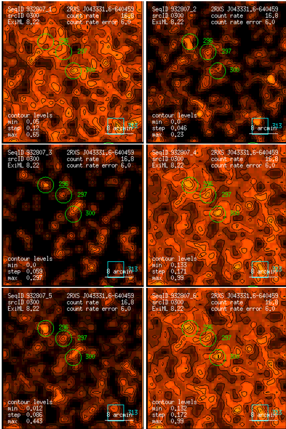
Figure 300: RASS 932807: detection 0300: band rate images, Gaussian filter: (1) PSPC channels 11 – 41, (2) 52 – 90, (3) 91 – 201, (4) 11 – 235, (5) 52 – 201, (6) 11 – 201. Broad band rates in counts/ks. Band rate contour levels in counts/ks/arcmin 2 .
