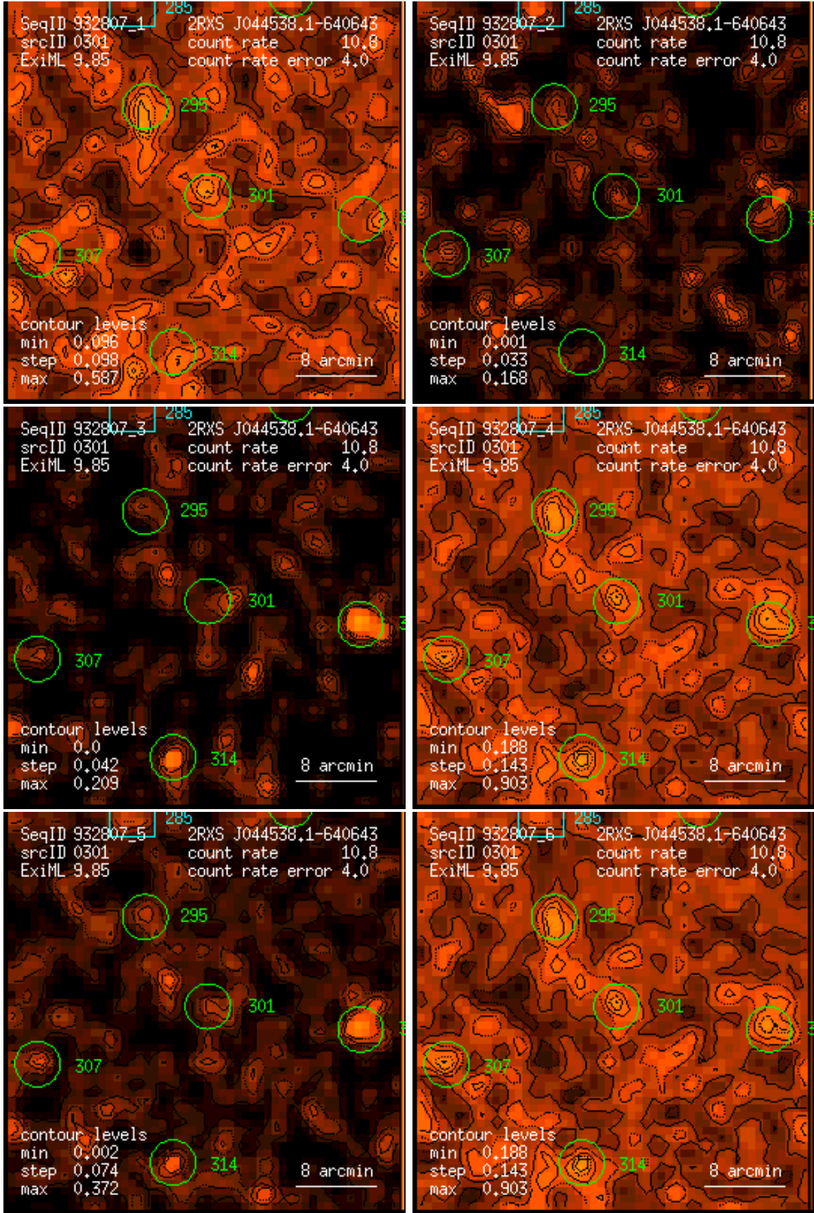
Figure 301: RASS 932807: detection 0301: band rate images, Gaussian filter: (1) PSPC channels 11 – 41, (2) 52 – 90, (3) 91 – 201, (4) 11 – 235, (5) 52 – 201, (6) 11 – 201. Broad band rates in counts/ks. Band rate contour levels in counts/ks/arcmin 2 .
