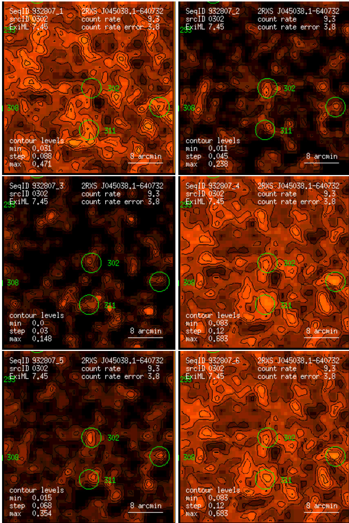
Figure 302: RASS 932807: detection 0302: band rate images, Gaussian filter: (1) PSPC channels 11 – 41, (2) 52 – 90, (3) 91 – 201, (4) 11 – 235, (5) 52 – 201, (6) 11 – 201. Broad band rates in counts/ks. Band rate contour levels in counts/ks/arcmin 2 .
