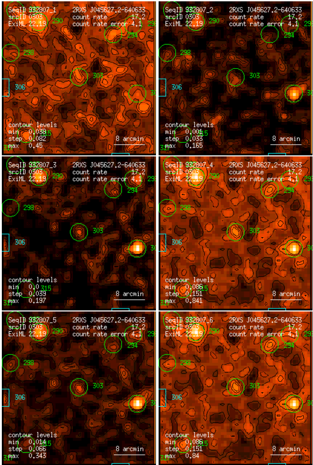
Figure 303: RASS 932807: detection 0303: band rate images, Gaussian filter: (1) PSPC channels 11 – 41, (2) 52 – 90, (3) 91 – 201, (4) 11 – 235, (5) 52 – 201, (6) 11 – 201. Broad band rates in counts/ks. Band rate contour levels in counts/ks/arcmin 2 .
