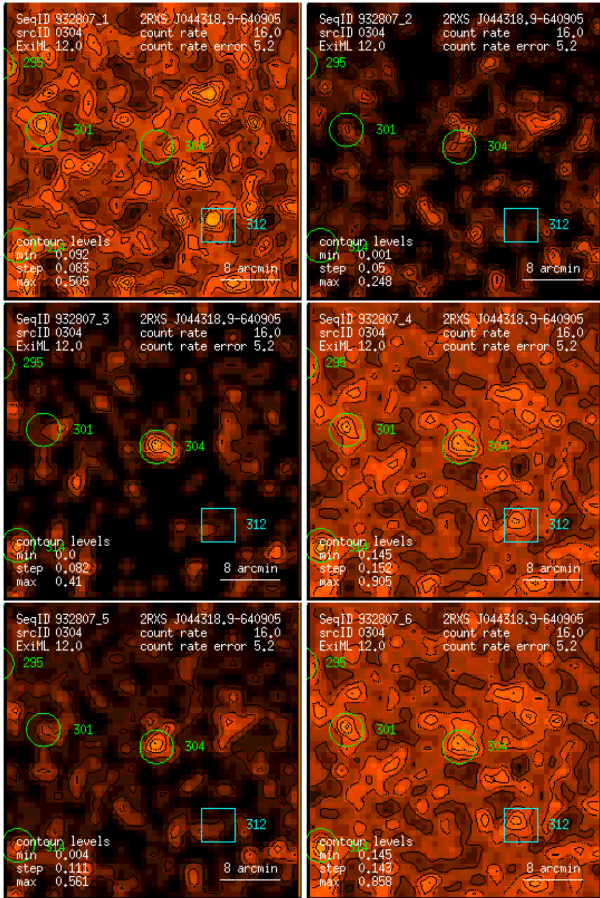
Figure 304: RASS 932807: detection 0304: band rate images, Gaussian filter: (1) PSPC channels 11 – 41, (2) 52 – 90, (3) 91 – 201, (4) 11 – 235, (5) 52 – 201, (6) 11 – 201. Broad band rates in counts/ks. Band rate contour levels in counts/ks/arcmin 2 .
