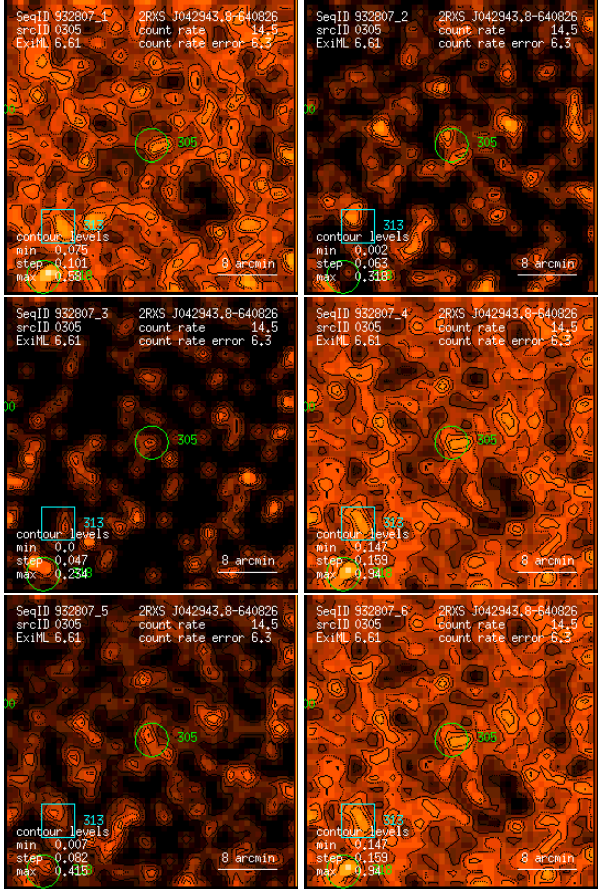
Figure 305: RASS 932807: detection 0305: band rate images, Gaussian filter: (1) PSPC channels 11 – 41, (2) 52 – 90, (3) 91 – 201, (4) 11 – 235, (5) 52 – 201, (6) 11 – 201. Broad band rates in counts/ks. Band rate contour levels in counts/ks/arcmin 2 .
