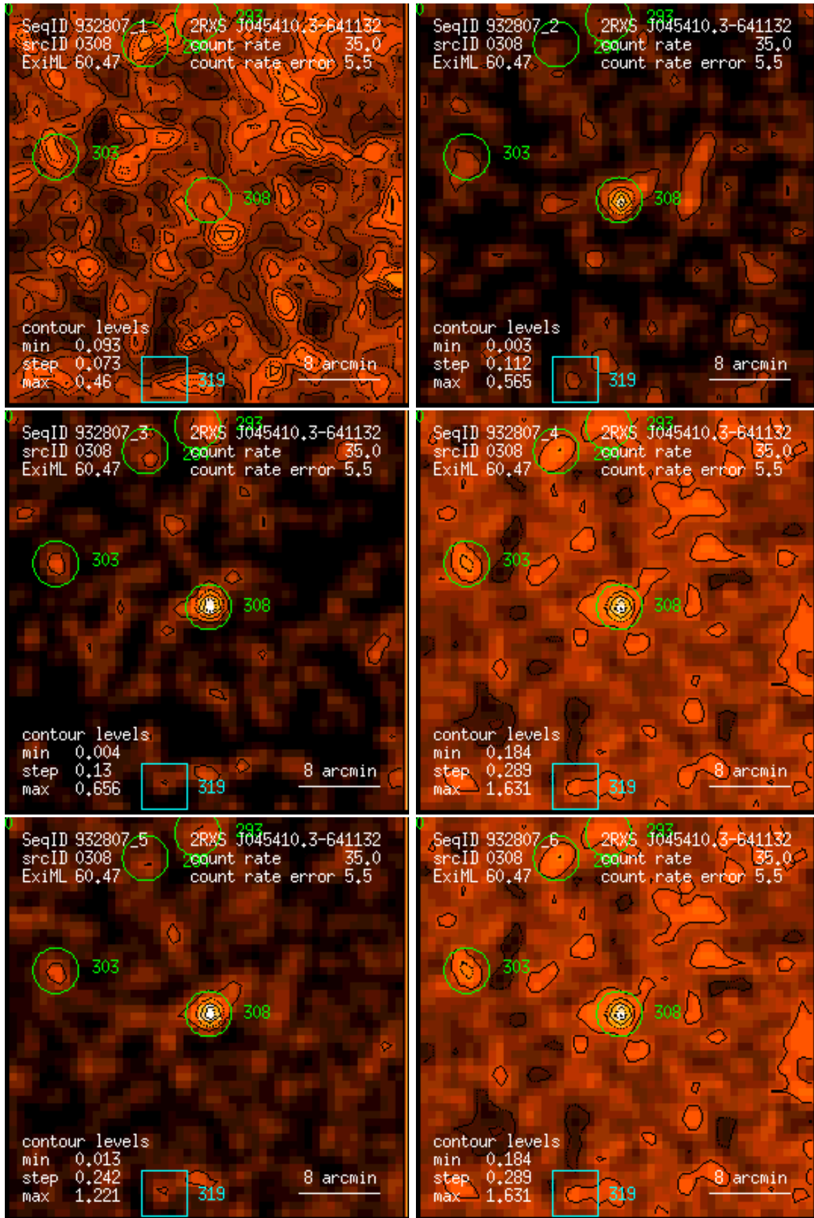
Figure 308: RASS 932807: detection 0308: band rate images, Gaussian filter: (1) PSPC channels 11 – 41, (2) 52 – 90, (3) 91 – 201, (4) 11 – 235, (5) 52 – 201, (6) 11 – 201. Broad band rates in counts/ks. Band rate contour levels in counts/ks/arcmin 2 .
