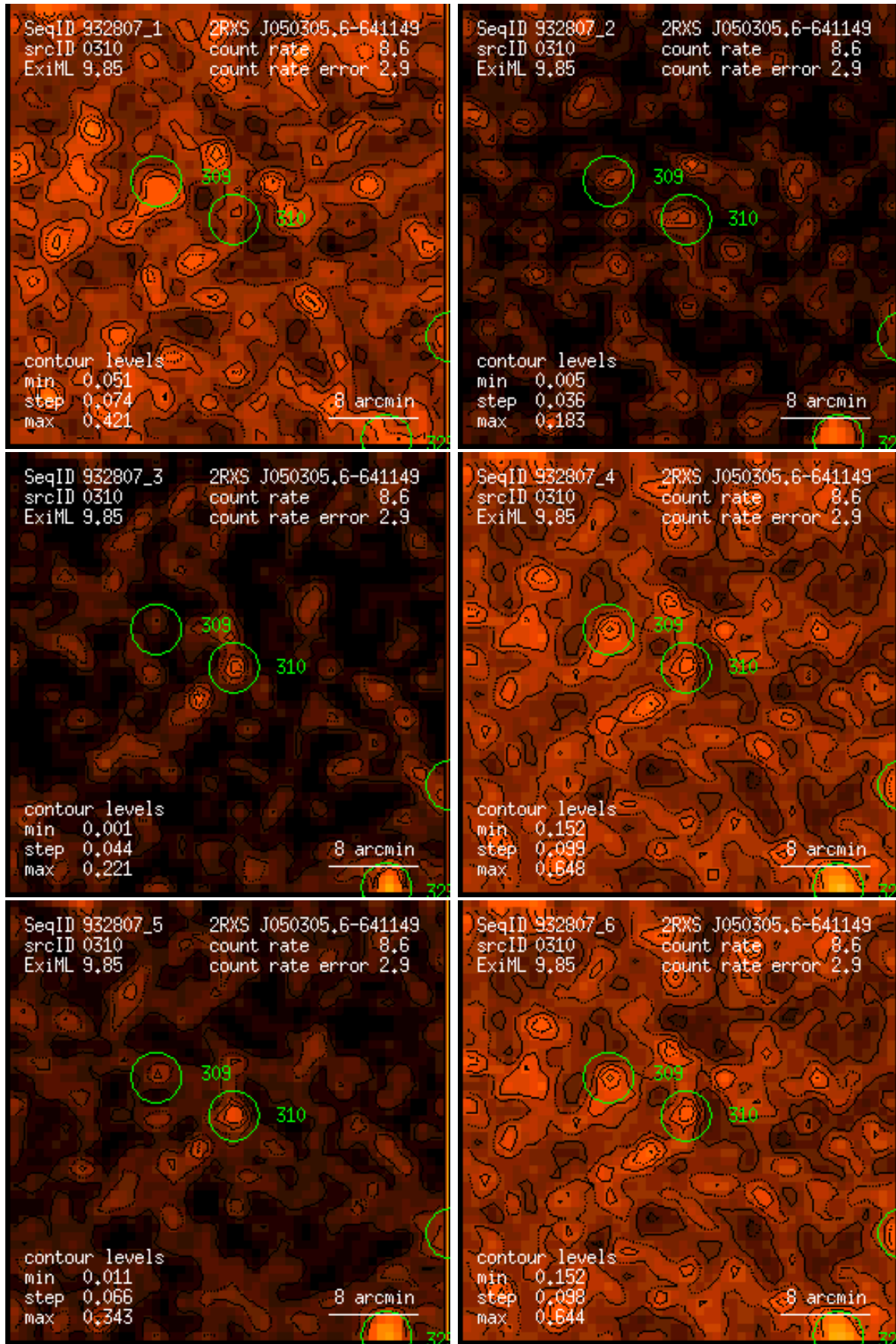
Figure 310: RASS 932807: detection 0310: band rate images, Gaussian filter: (1) PSPC channels 11 – 41, (2) 52 – 90, (3) 91 – 201, (4) 11 – 235, (5) 52 – 201, (6) 11 – 201. Broad band rates in counts/ks. Band rate contour levels in counts/ks/arcmin 2 .
