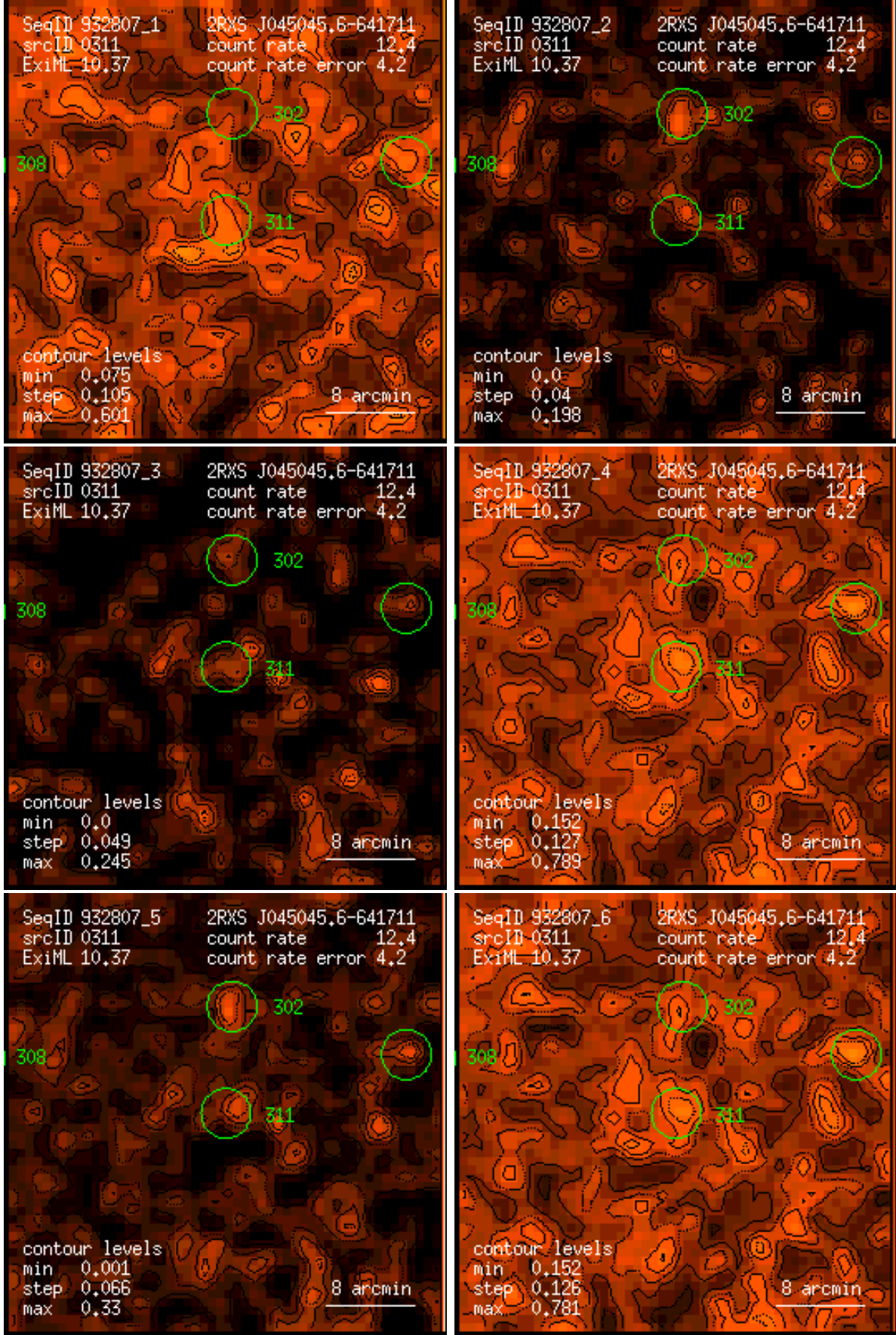
Figure 311: RASS 932807: detection 0311: band rate images, Gaussian filter: (1) PSPC channels 11 – 41, (2) 52 – 90, (3) 91 – 201, (4) 11 – 235, (5) 52 – 201, (6) 11 – 201. Broad band rates in counts/ks. Band rate contour levels in counts/ks/arcmin 2 .
